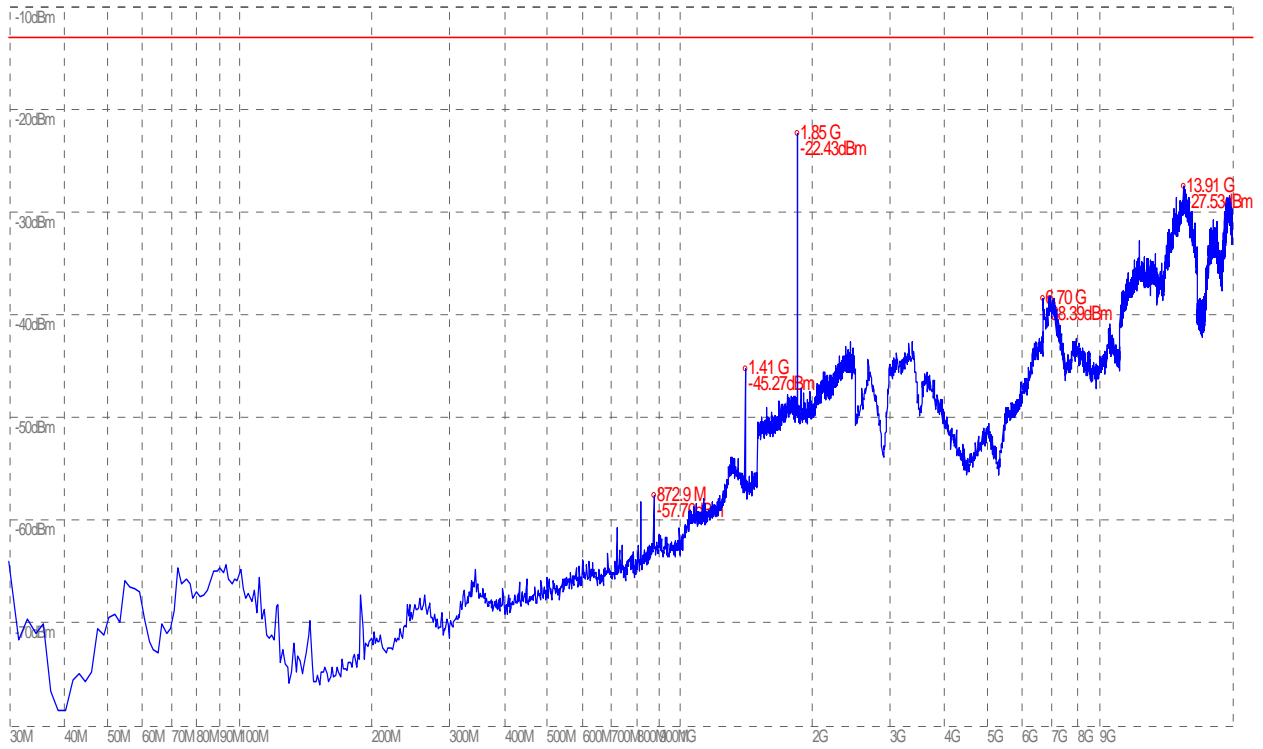
(Plot D.1: GSM 1900MHz Channel = 512, Test Antenna Horizontal)
