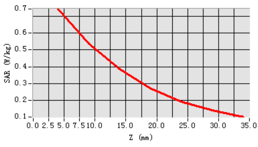
SAR, Z Axis Scan (X = 0, Y = -23)
