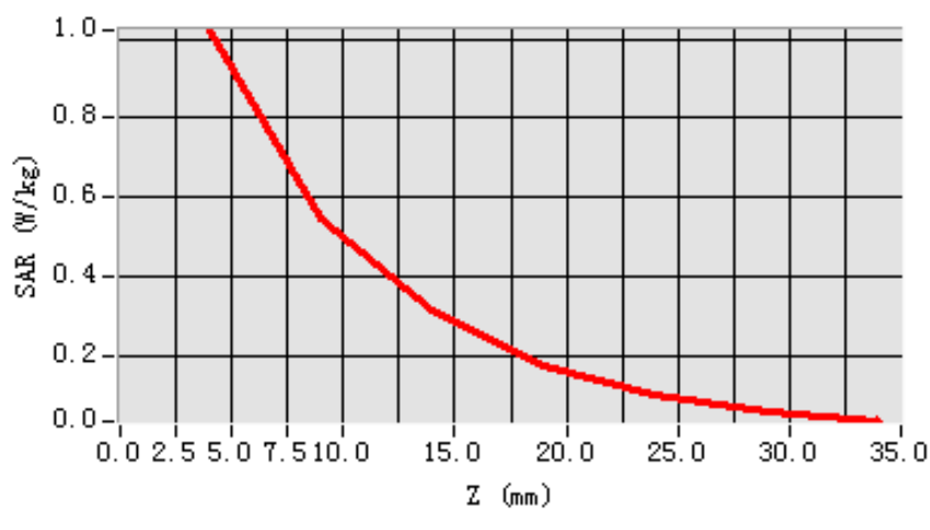
SAR, Z Axis Scan (X = -24, Y = 8)
