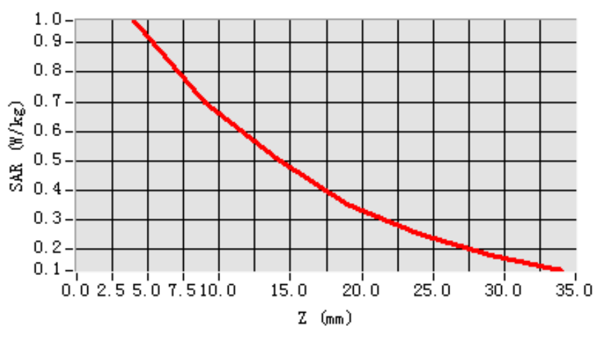
SAR, Z Axis Scan (X = -48, Y = -32)
