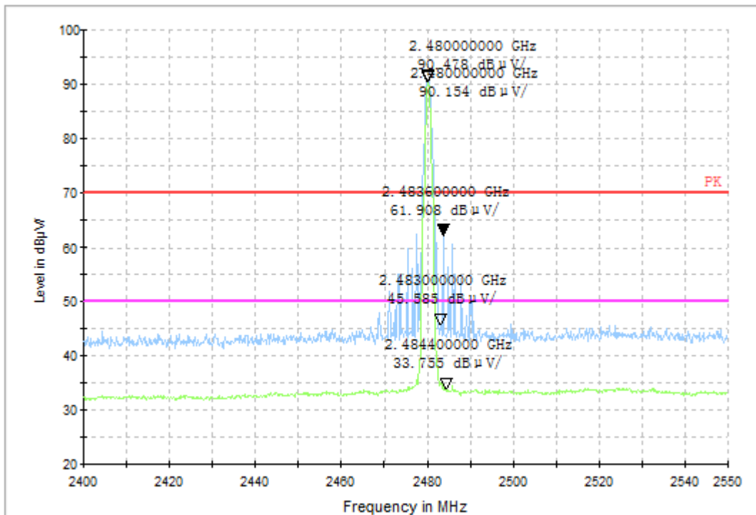
GFSK Channel 78, fixed mode, right band-edge
