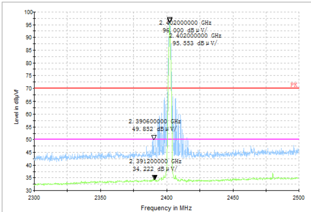
GFSK Channel 0, fixed mode, left band-edge
