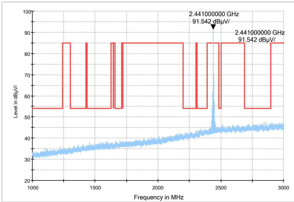
GFSK DH5 Channel 39 1-3GHz
