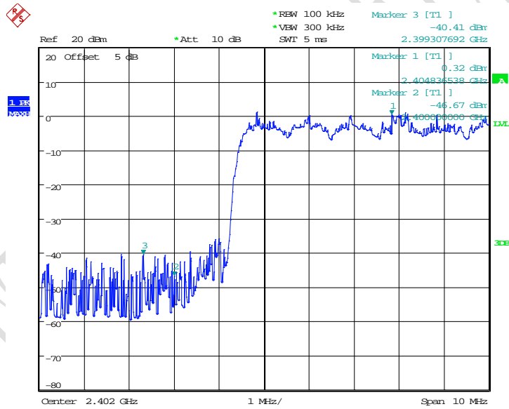
8DPSK Channel 0, fixed mode, left band-edge
