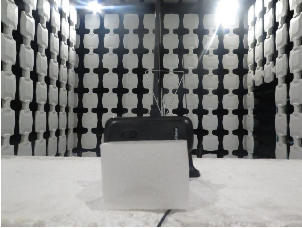
Pic3. RSE and EIRP/ERP
