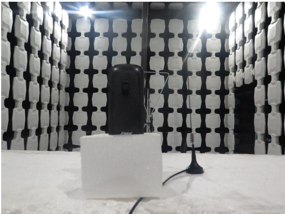
Pic2. RSE and EIRP/ERP
