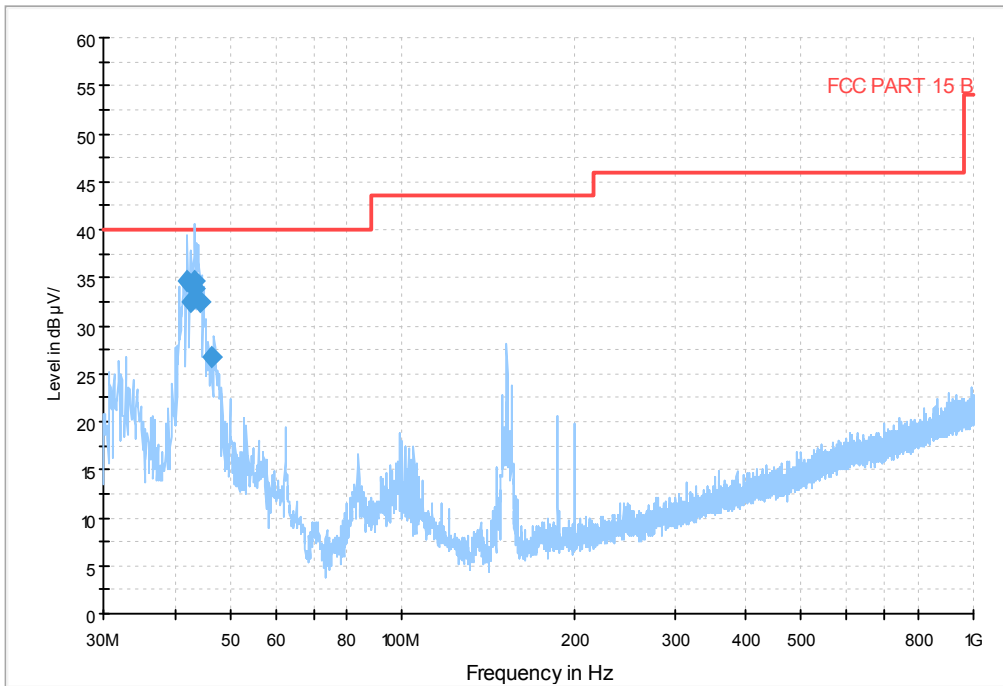
GFSK DH5 Channel 39 30MHz-1GHz
