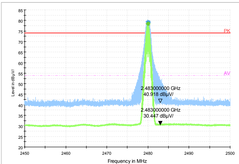
BAND EDGERE 1GHz-3GHz 2483.5-2500
