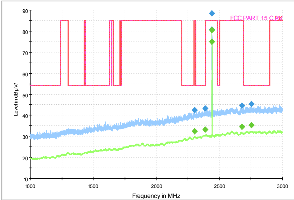
GFSK DH5 Channel 39 1-3GHz
