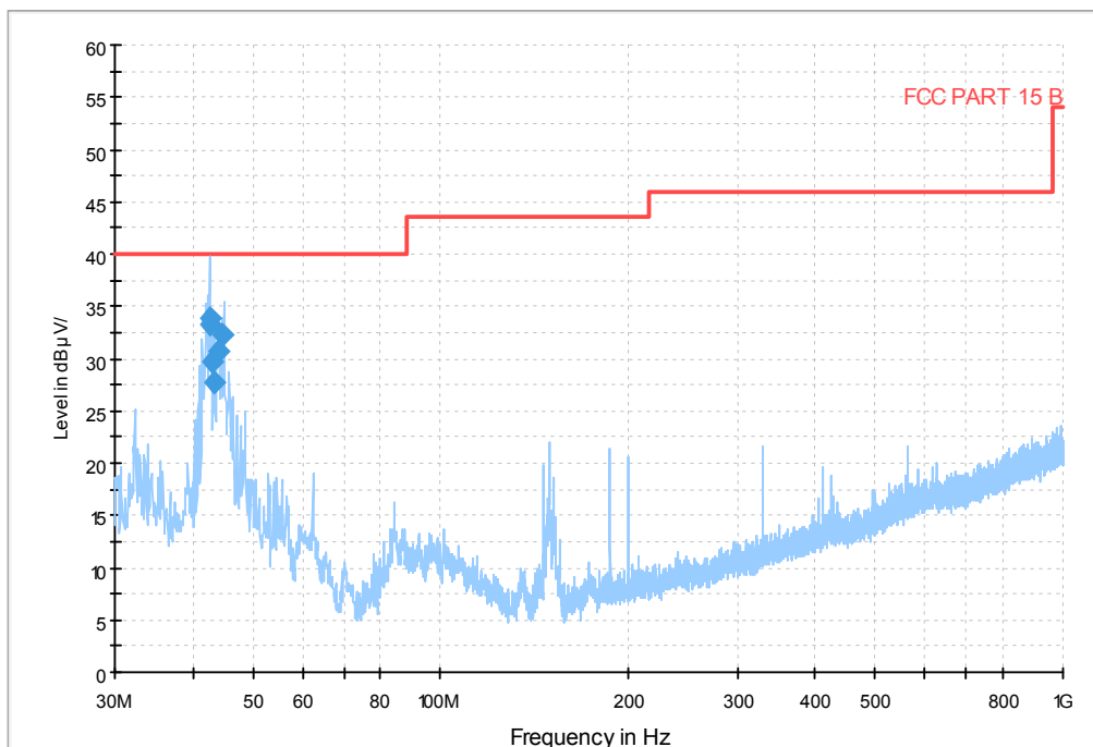
GFSK DH5 Channel 78 30MHz-1GHz
