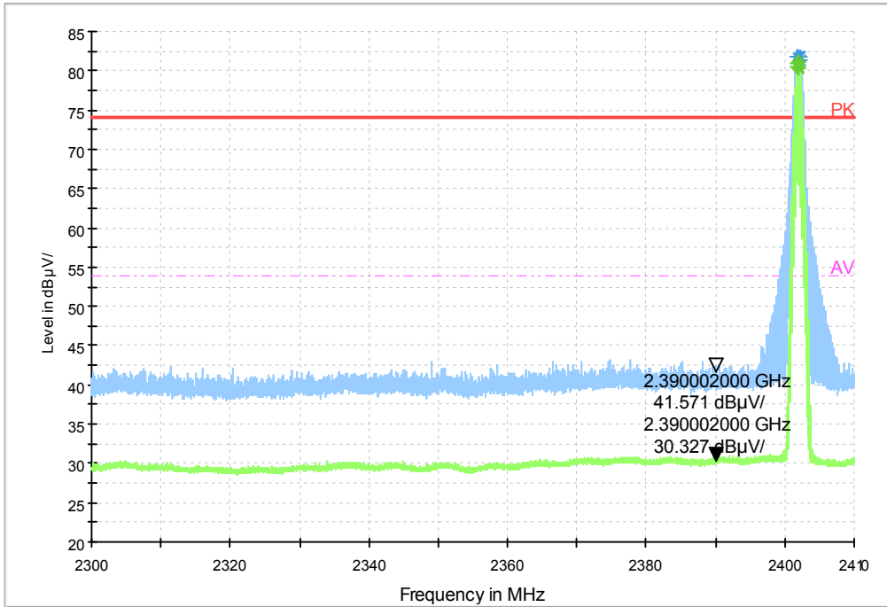
BAND EDGERE 1GHz-3GHz 2300-2390
