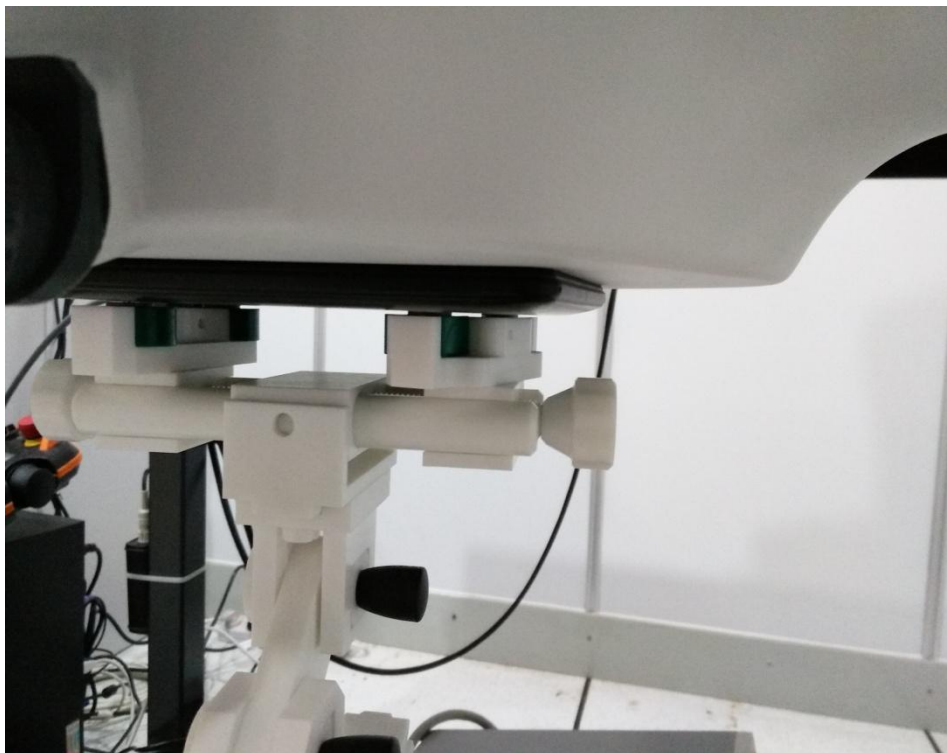
Fig.6 Body (Face upside,0mm separation)
