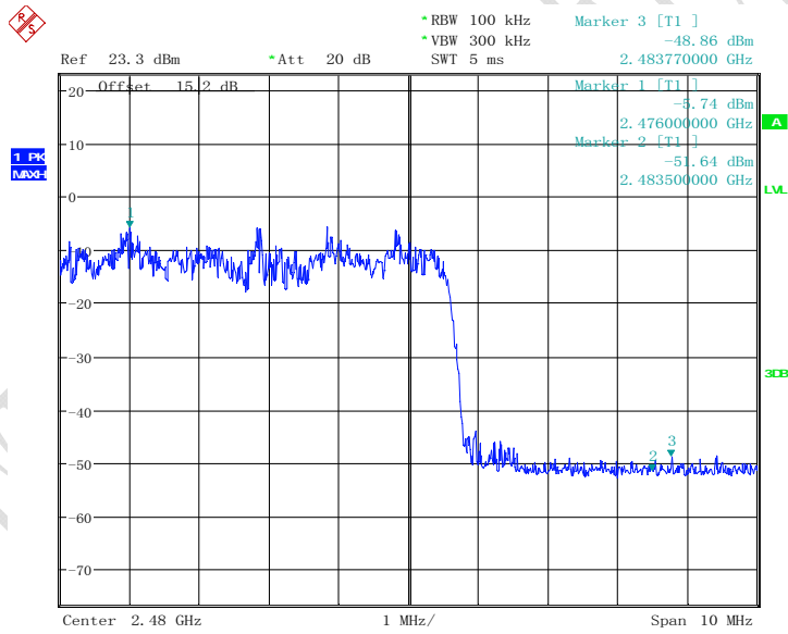
Pi/4 DQPSK Channel 78, fixed mode, right band-edge
