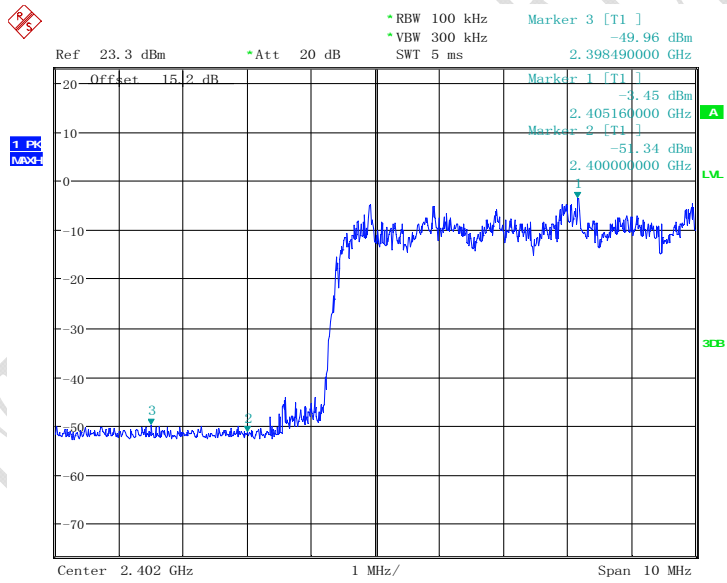
8DPSK Channel 0, fixed mode, left band-edge
