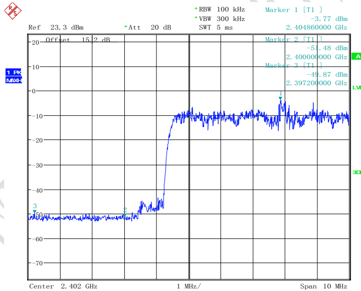
Pi/4 DQPSK Channel 0, fixed mode, left band-edge
