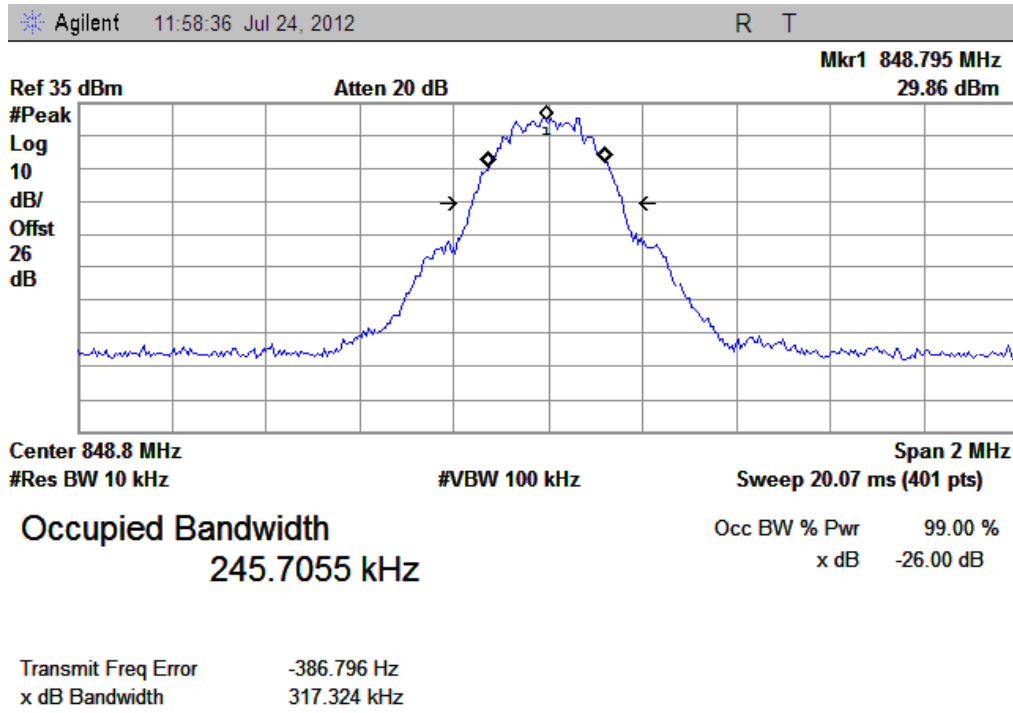
(Plot C: GSM 850MHz Channel = 251)
