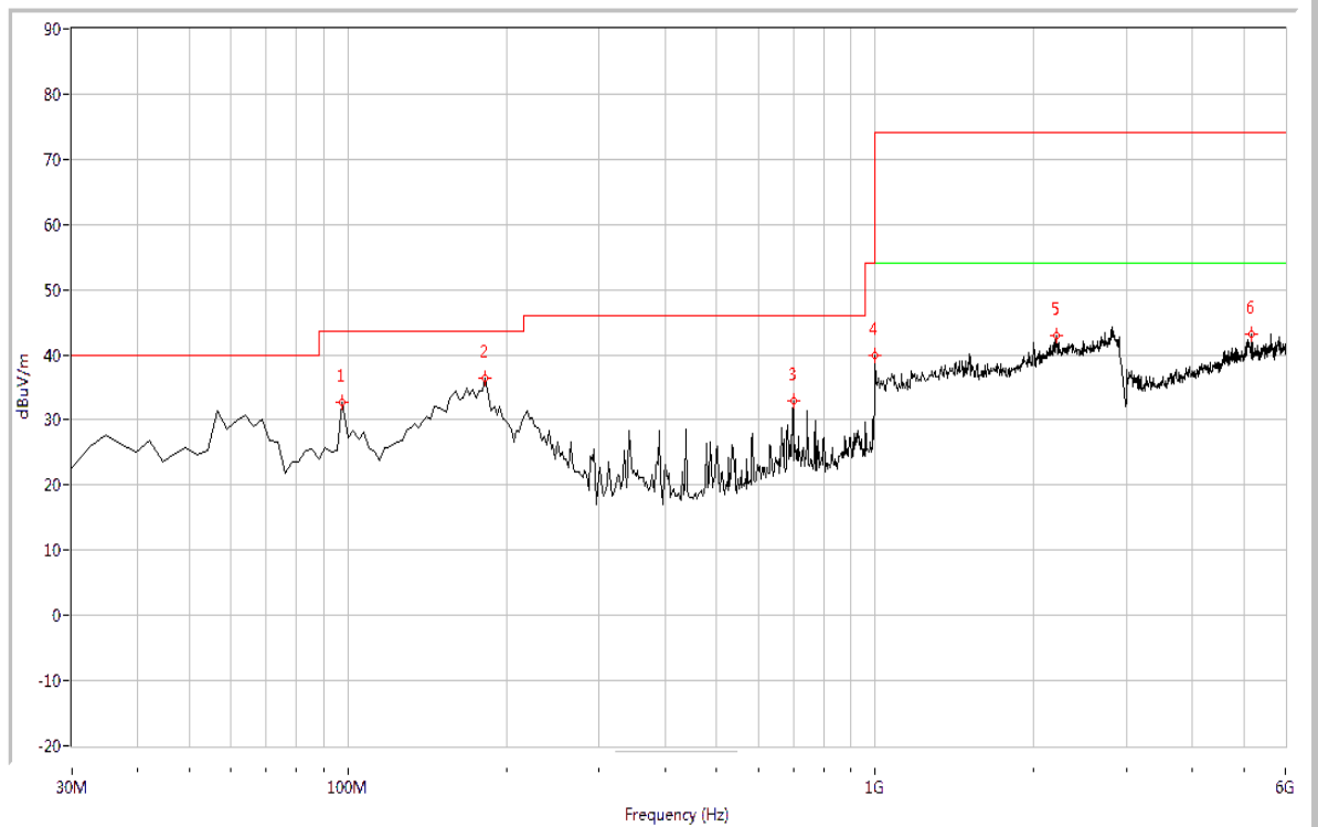
(Plot B: 30MHz – 6GHz, Test Antenna Vertical)
