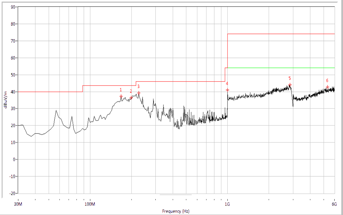
(Plot C: 30MHz – 6GHz, Test Antenna Horizontal)
