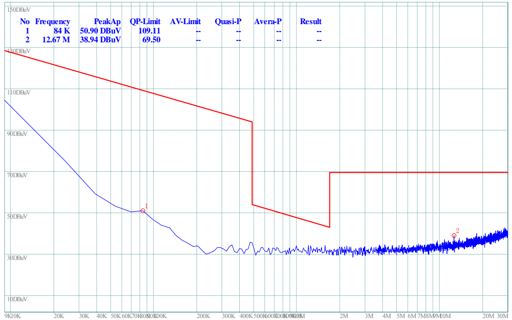
(Plot G.1: 9kHz to 30MHz)
