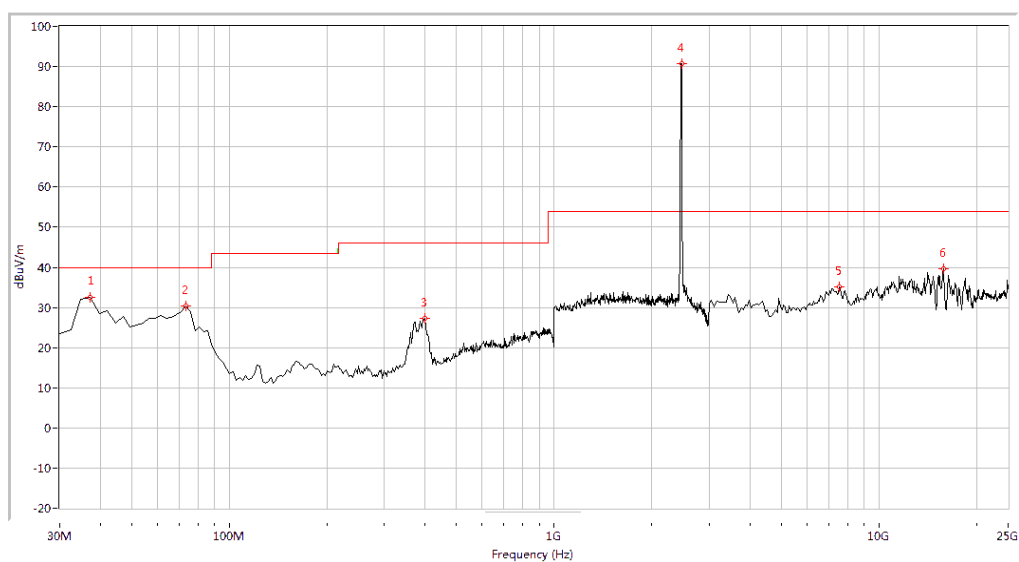
(Plot C.2: Antenna Horizontal, 30MHz to 25GHz)
