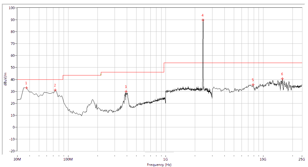
(Plot D.2: Antenna Horizontal, 30MHz to 25GHz)
