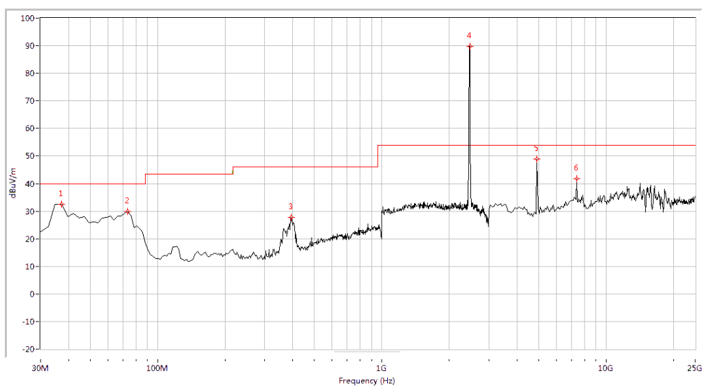
(Plot F.2: Antenna Horizontal, 30MHz to 25GHz)
