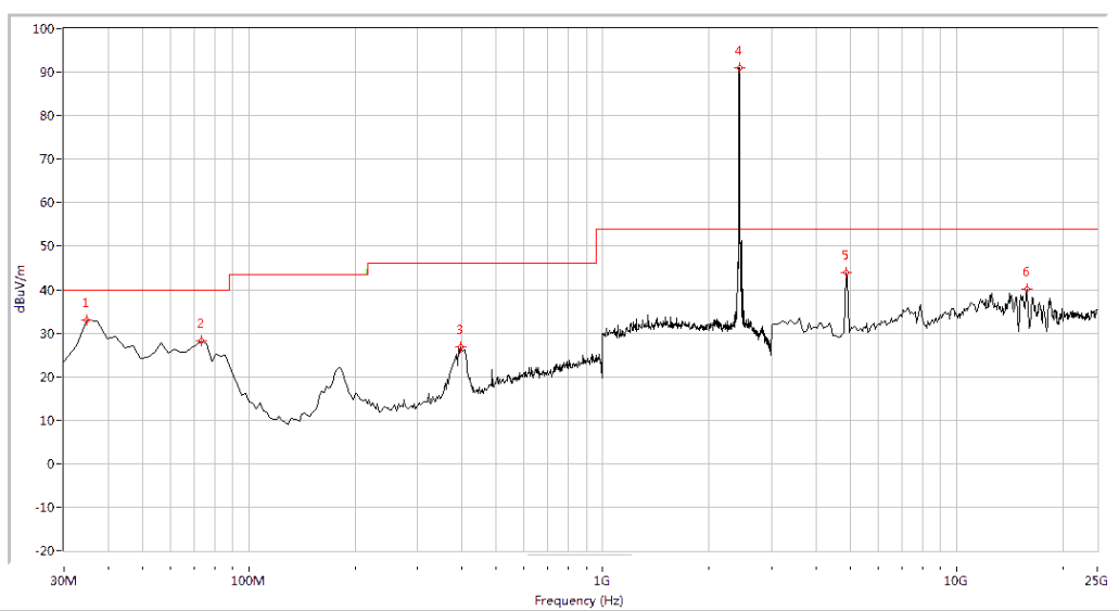
(Plot K.2: Antenna Horizontal, 30MHz to 25GHz)
