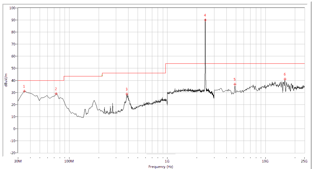
(Plot H.2: Antenna Horizontal, 30MHz to 25GHz)
