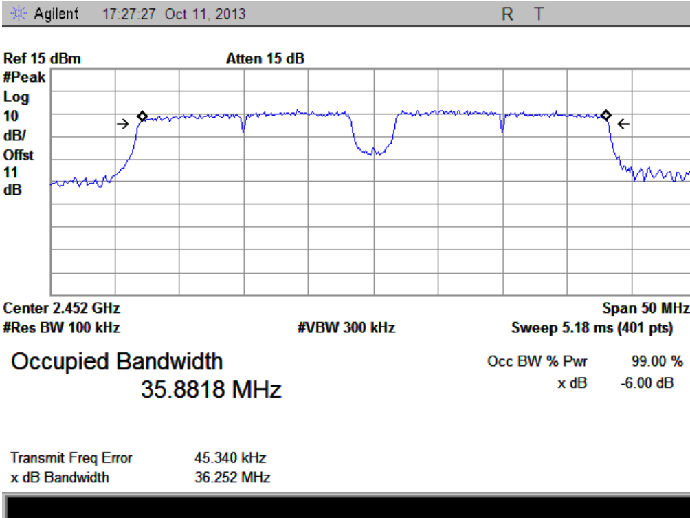
(Plot I: Channel 11: 2452MHz @ 802.11n-40)
