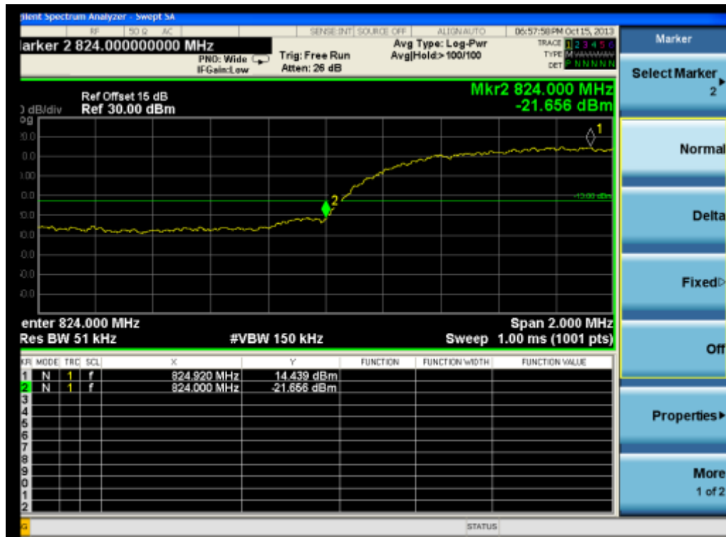
(Plot U: HSPA+ 850 Channel = 4132)
