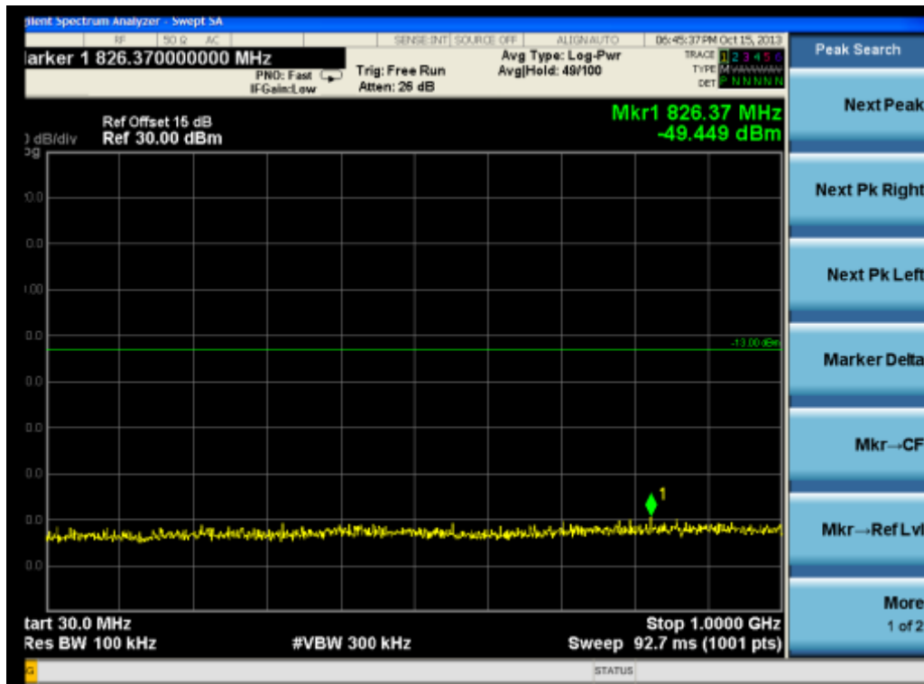
(Plot J 1: HSUPA1900MHz Channel = 9262, 30MHz to 1GHz)
