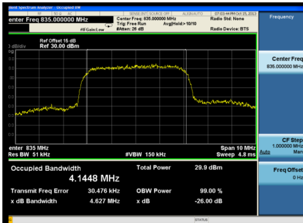
(Plot Z: HSPA+850 MHz Channel = 4175)
