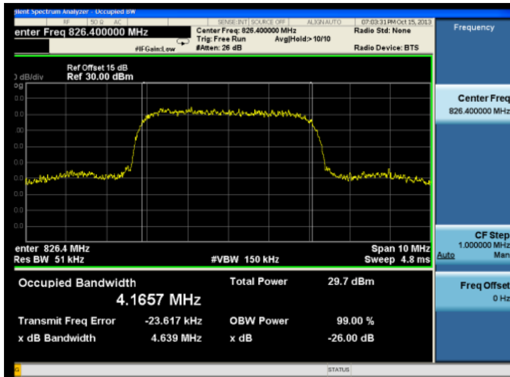
(Plot Y: HSPA+ 850 MHz Channel = 4132)
