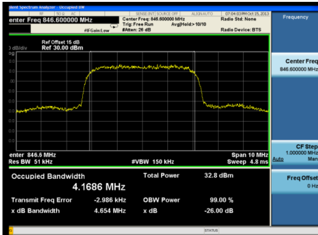
(Plot A1: HSPA+ 850 MHz Channel = 4233)
