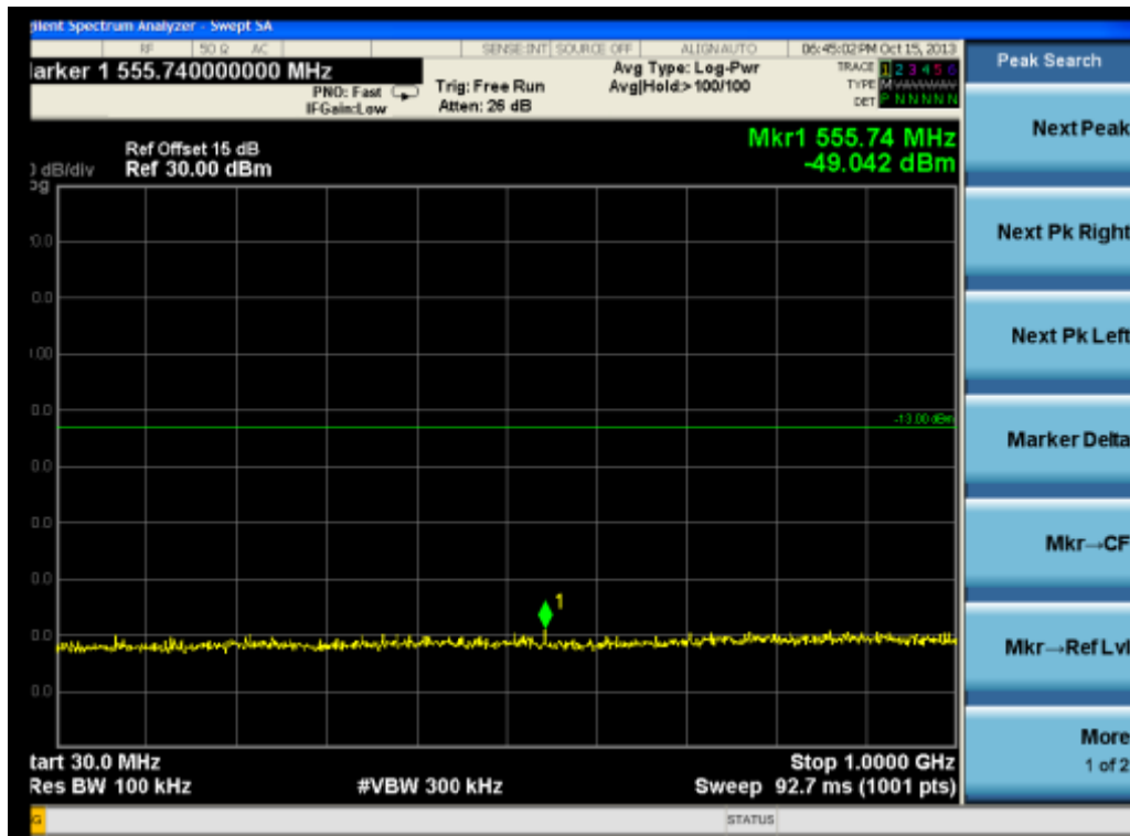
(Plot J 3: HSUPA1900MHz Channel = 9538, 30MHz to 1GHz)
