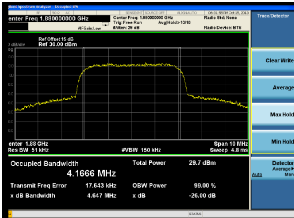
(Plot W: HSUPA1900 MHz Channel = 9400)
