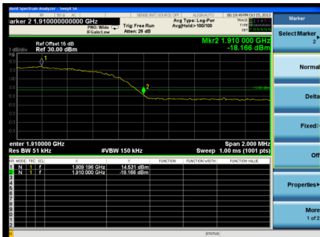
(Plot P: HSDPA 1900 Channel = 9538)
