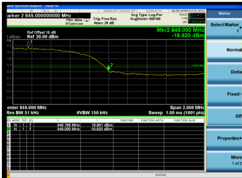
(Plot V: HSPA+ 850 Channel = 4233)
