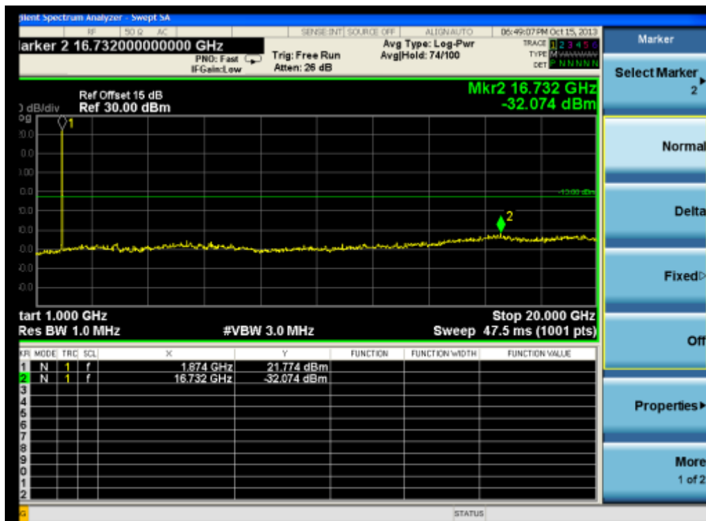
(Plot J2.1: HSUPA1900MHz Channel = 9400, 1GHz to 20GHz)
