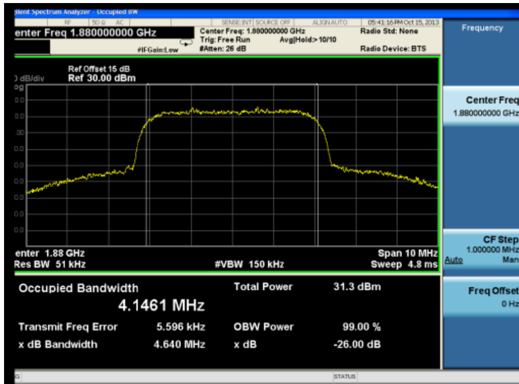
(Plot Q: HSDPA1900 MHz Channel = 9400)
