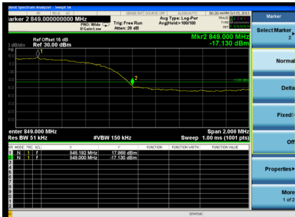
(Plot R: HSUPA850 Channel = 4233)
