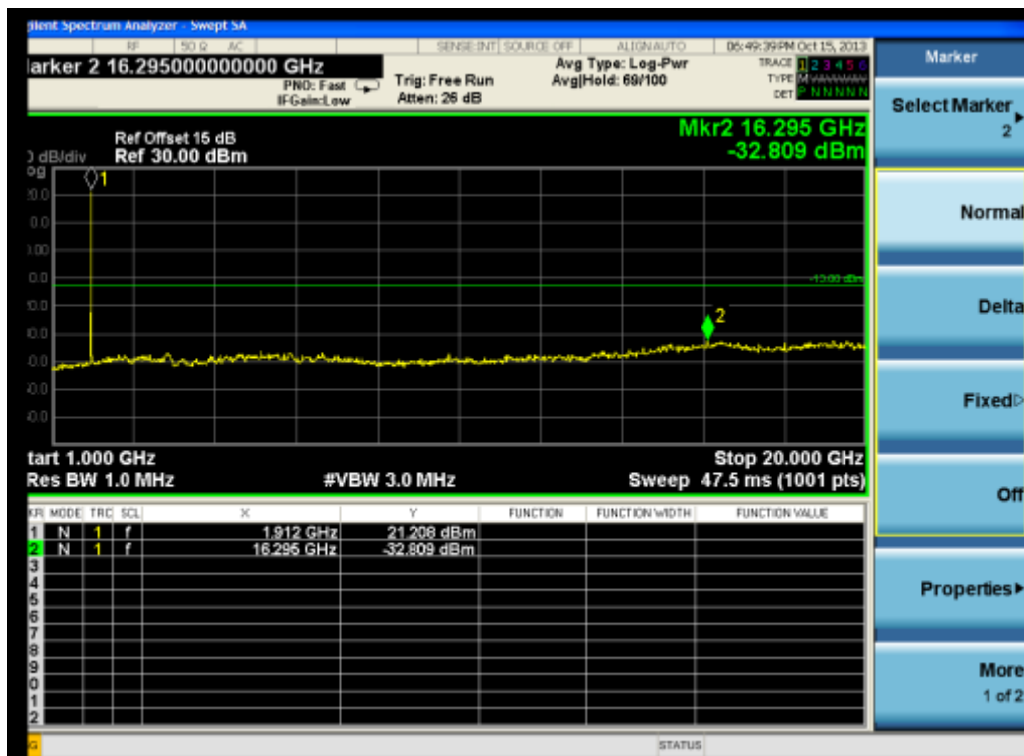
(Plot J3.1: HSUPA1900MHz Channel = 9538 1GHz to 20GHz)
