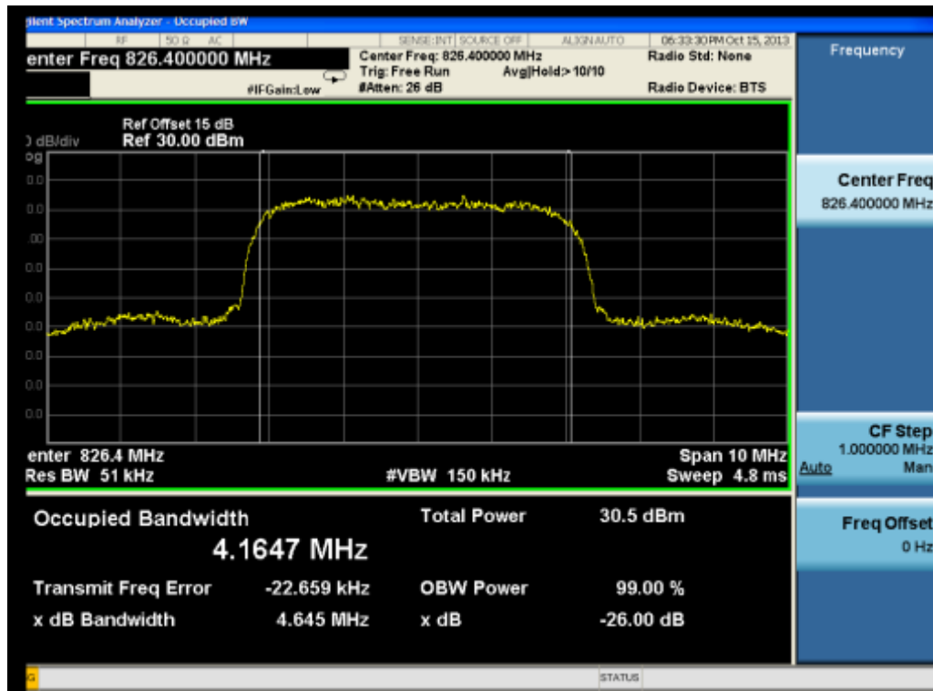
(Plot S: HSUPA850 MHz Channel = 4132)
