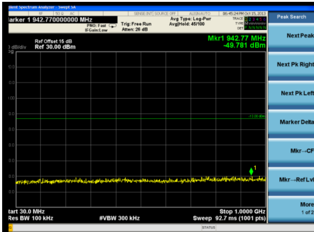
(Plot J 2: HSUPA1900MHz Channel = 9400, 30MHz to 1GHz)
