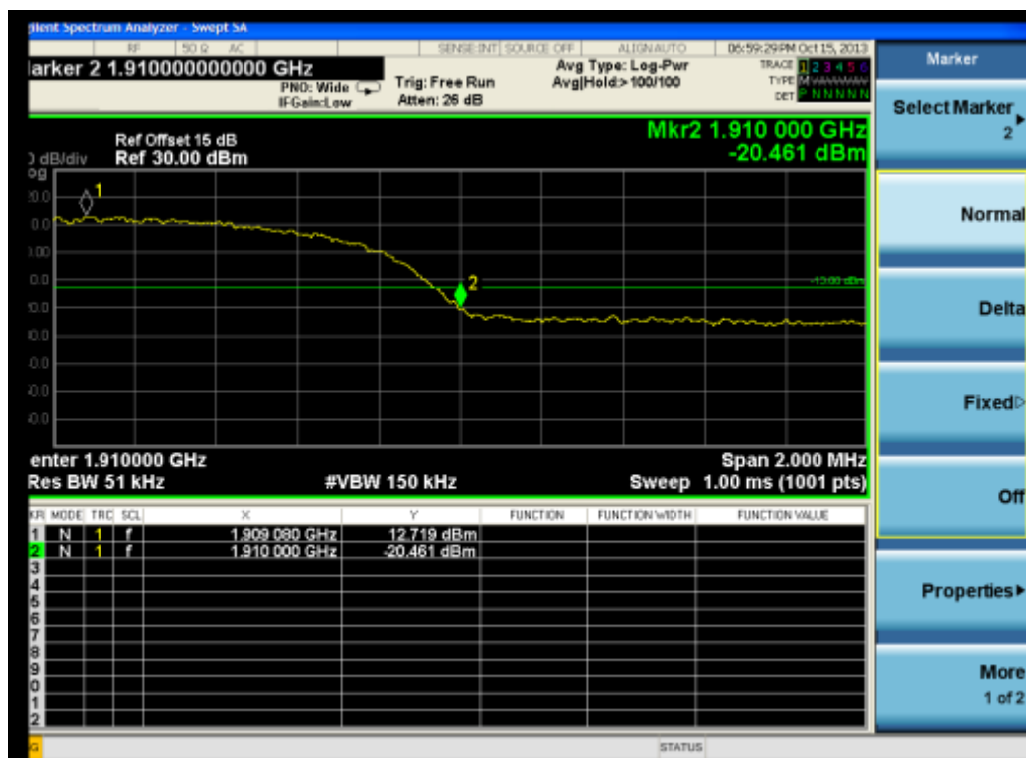
(Plot X: HSPA+ 1900 Channel = 9538)
