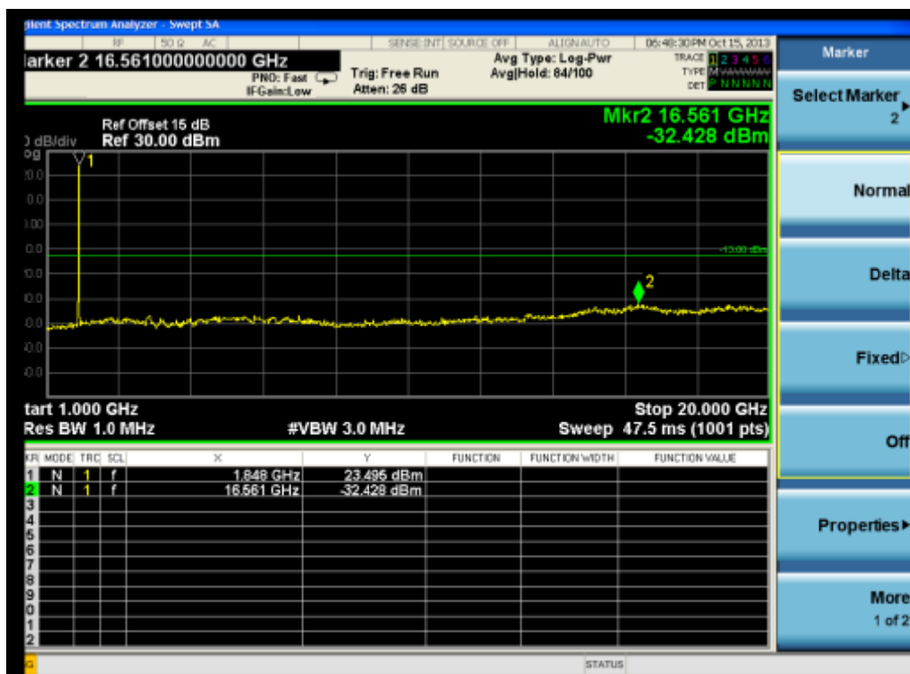
(Plot J1.1: HSUPA1900MHz Channel = 9262, 1GHz to 20GHz)
