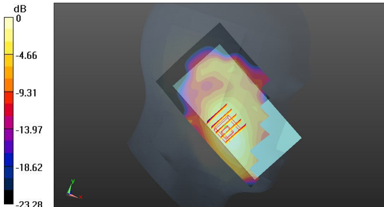
0 dB = 0.638 W/kg
