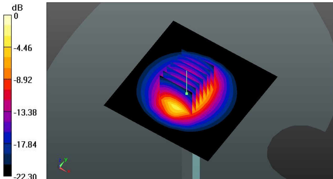
0 dB = 20.2 W/kg
