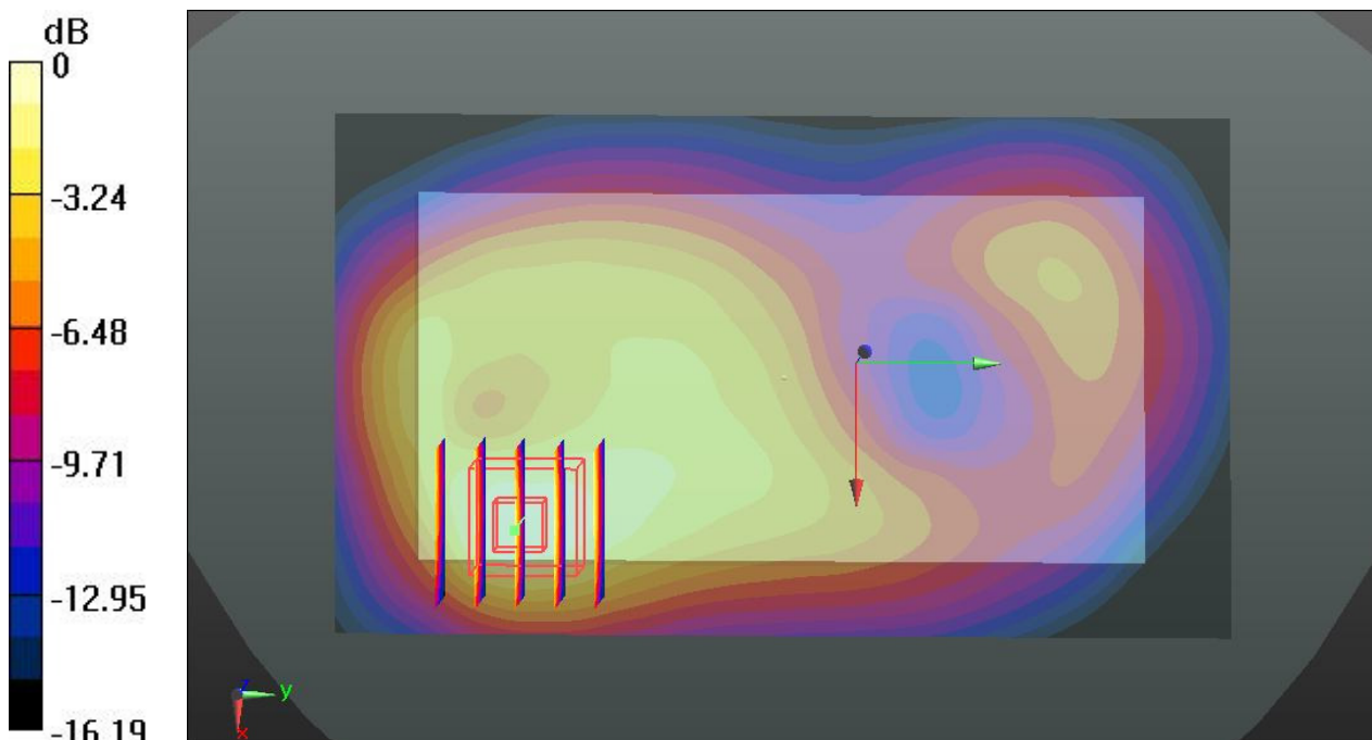
0 dB = 0.979 W/kg
