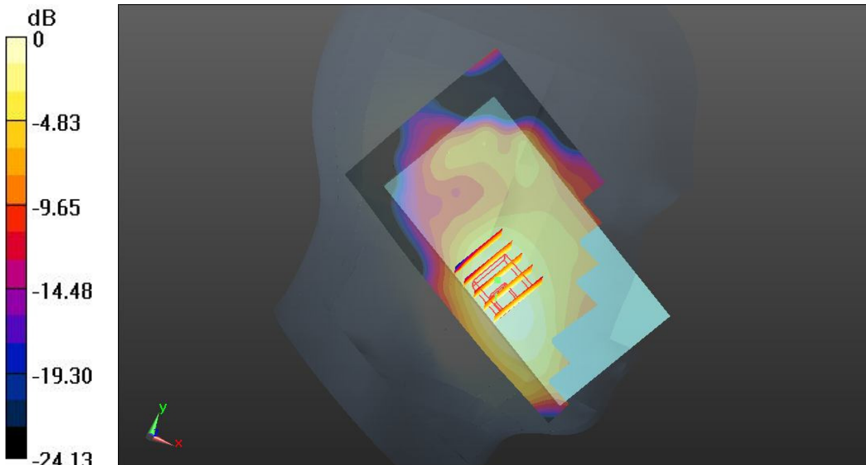
0 dB = 0.801 W/kg
