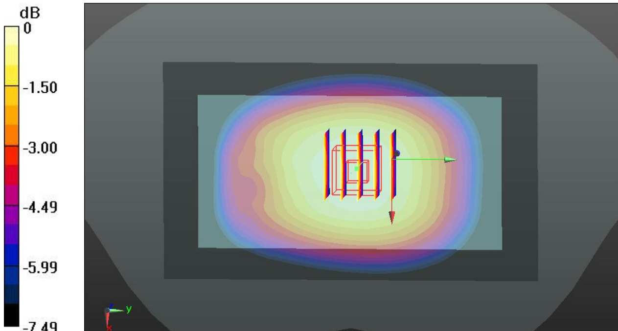
0 dB = 1.36 W/kg
