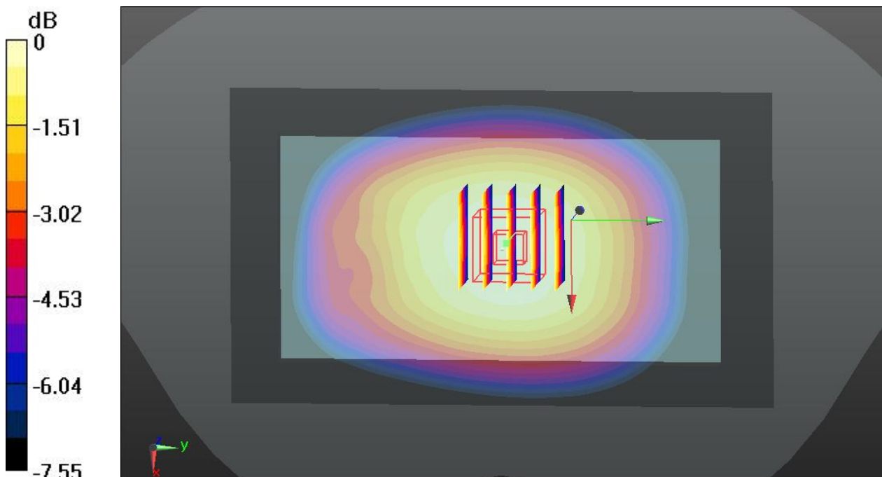
0 dB = 0.618 W/kg
