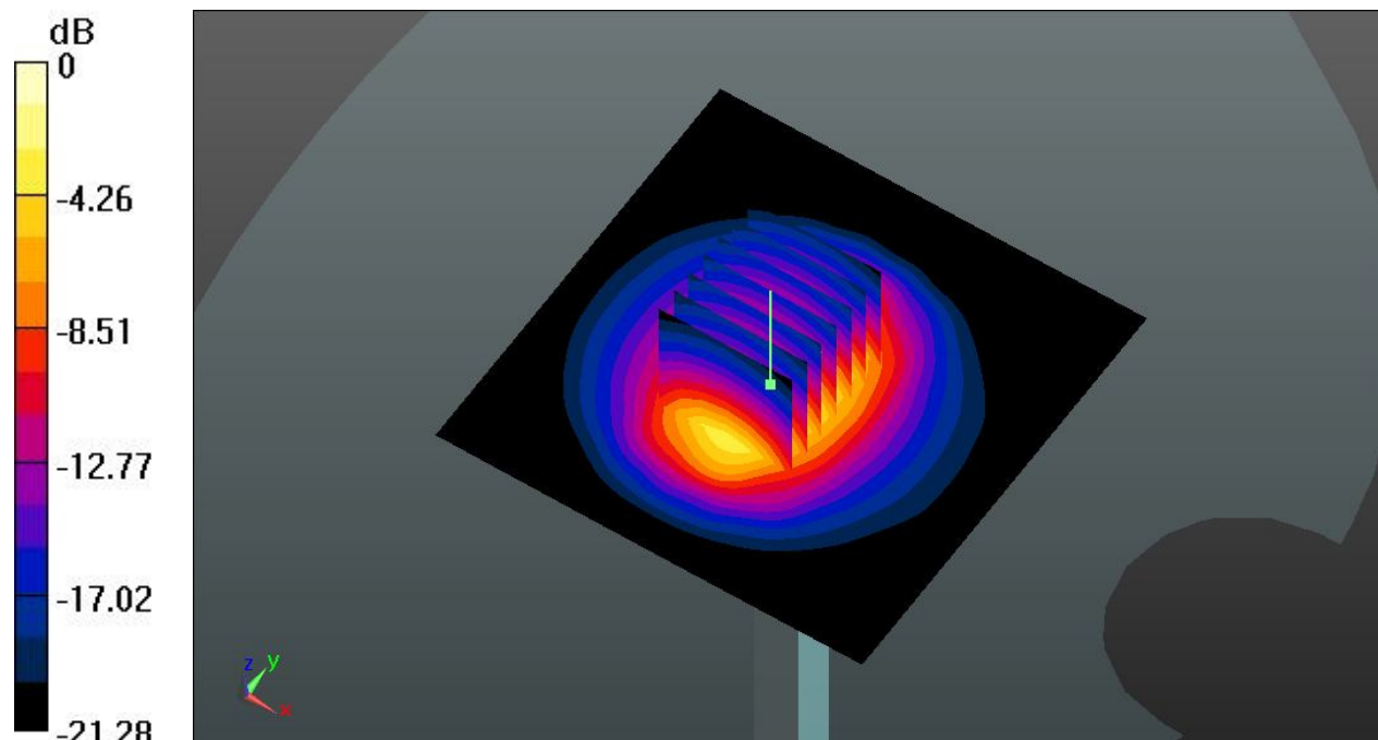
0 dB = 18.7 W/kg
