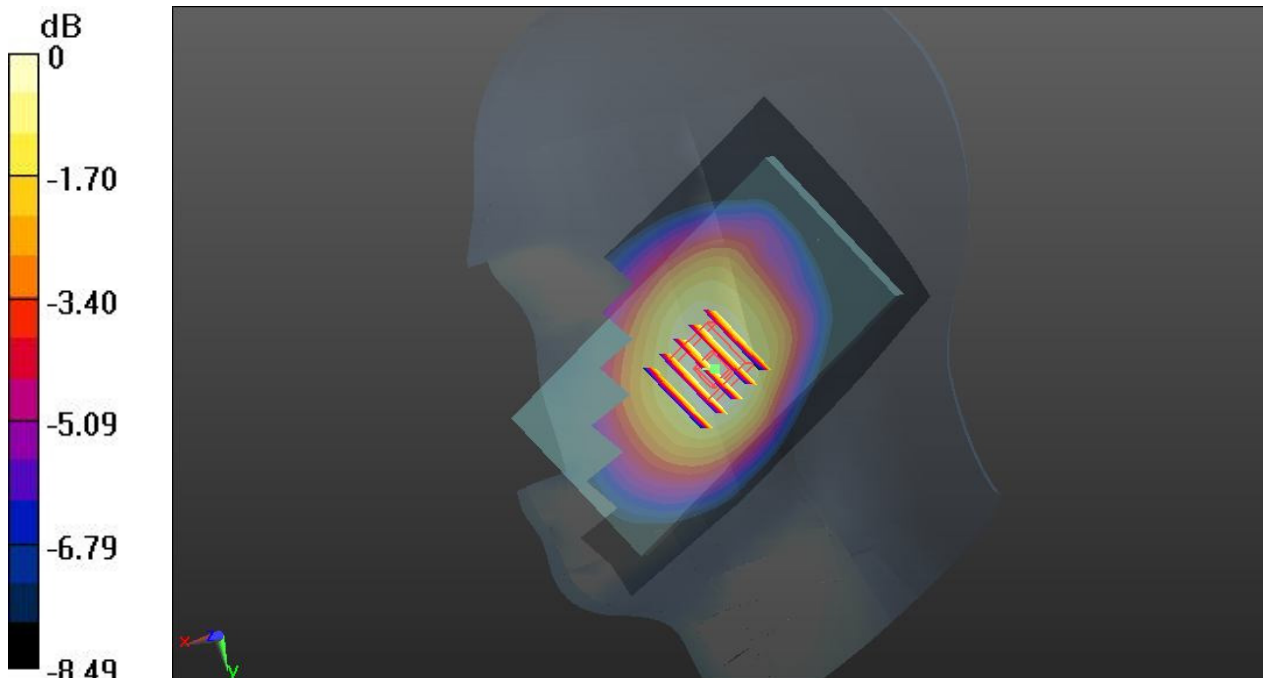
0 dB = 0.708 W/kg
