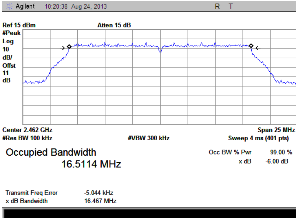
(Plot F: Channel 11: 2462MHz @ 802.11g)
