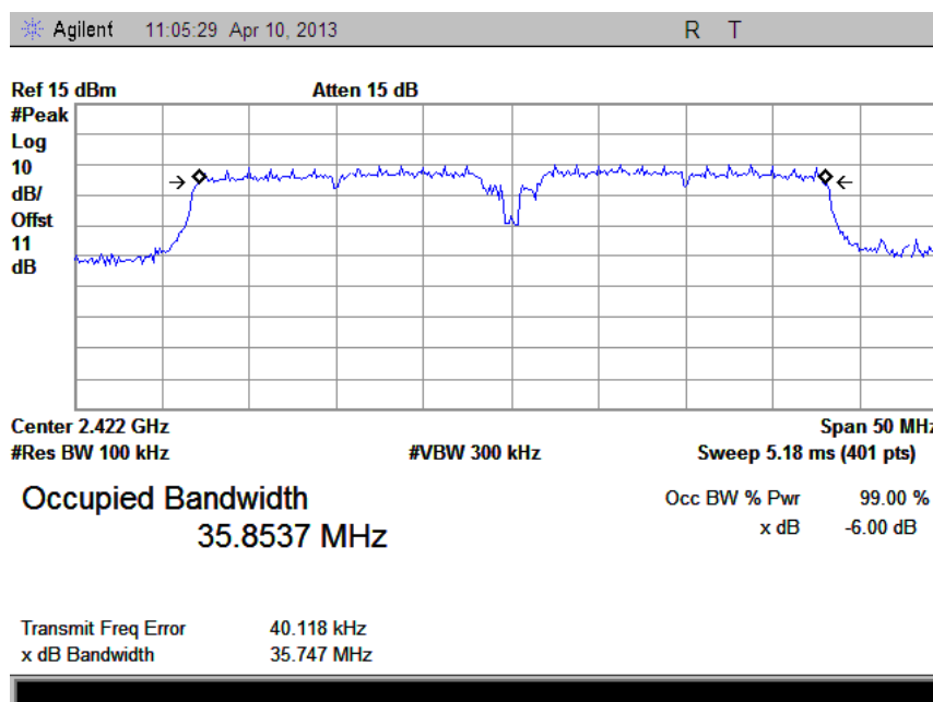
(Plot G: Channel 1: 2422MHz @ 802.11n-40)
