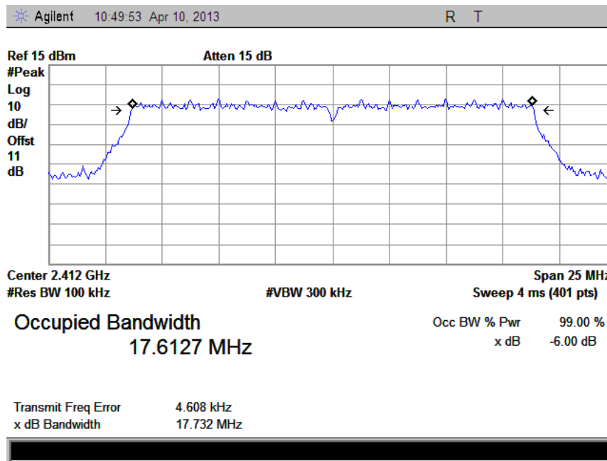
(Plot G: Channel 1: 2412MHz @ 802.11n-20)
