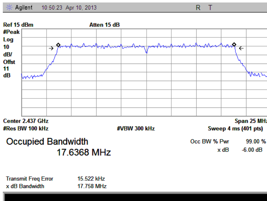
(Plot H: Channel 6: 2437MHz @ 802.11n-20)
