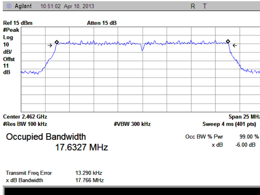
(Plot I: Channel 11: 2462MHz @ 802.11n-20)
