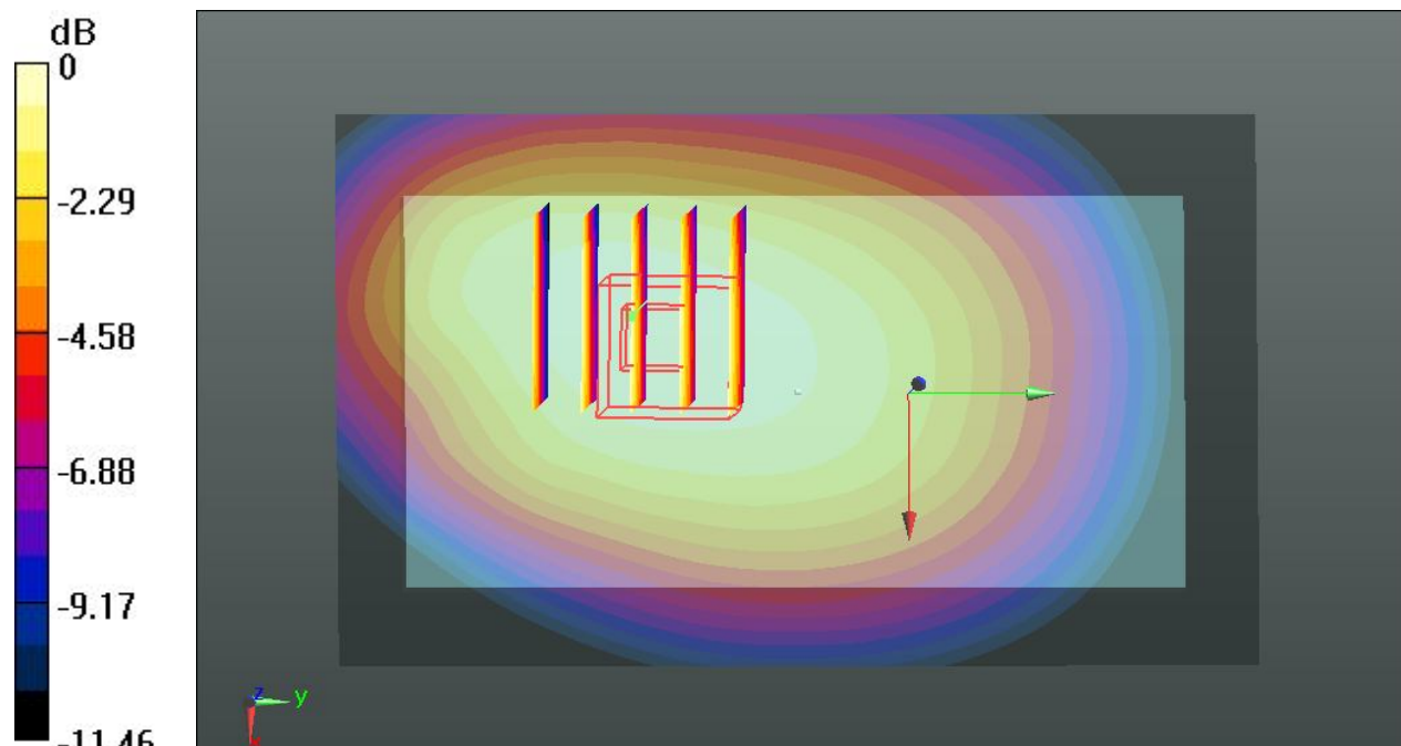
0 dB = 0.945 W/kg
