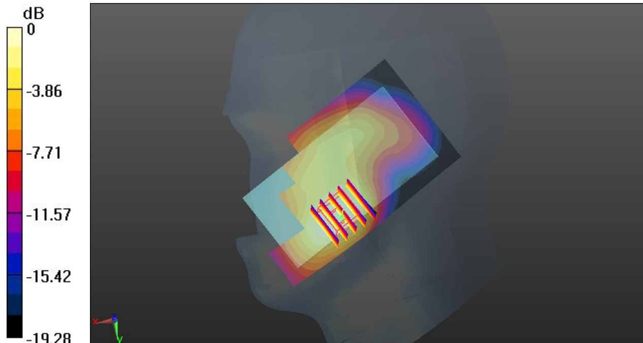
0 dB = 0.662 W/kg
