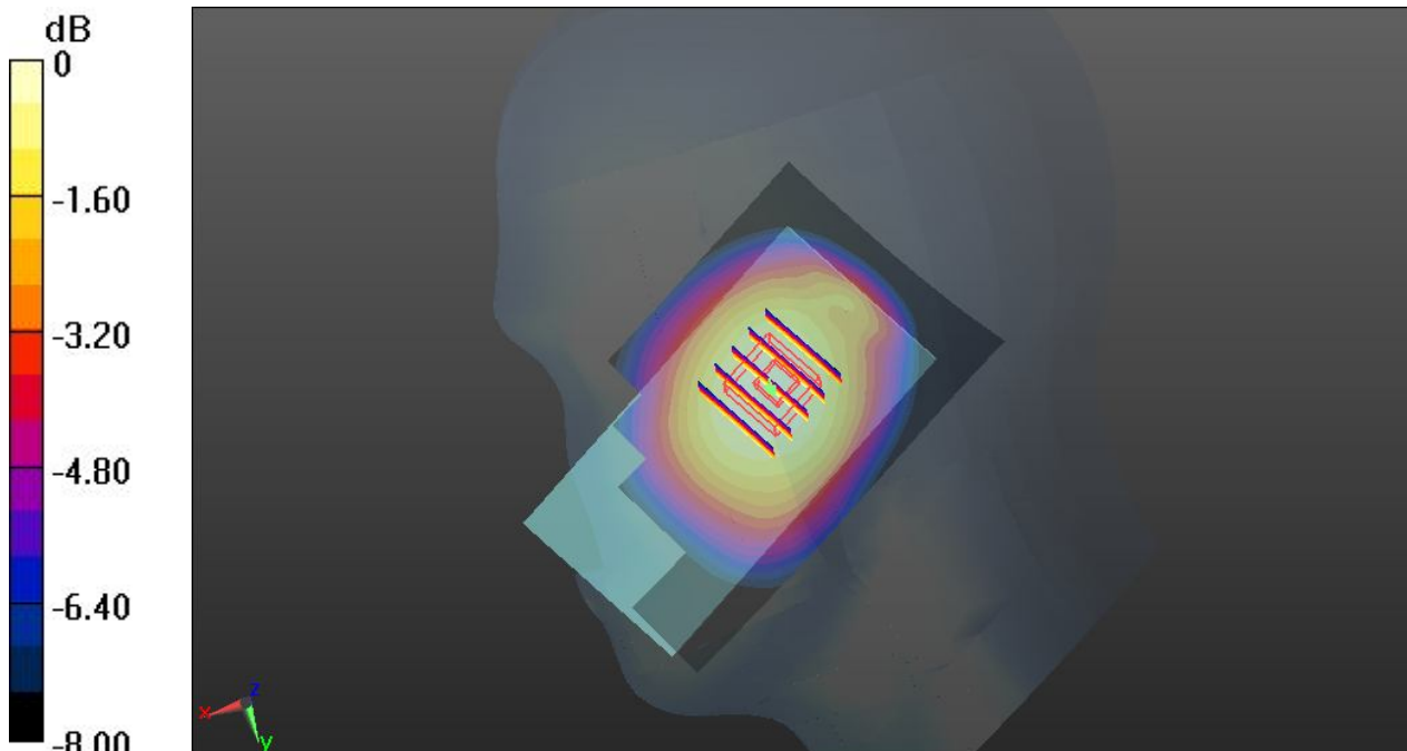
0 dB = 0.455 W/kg
