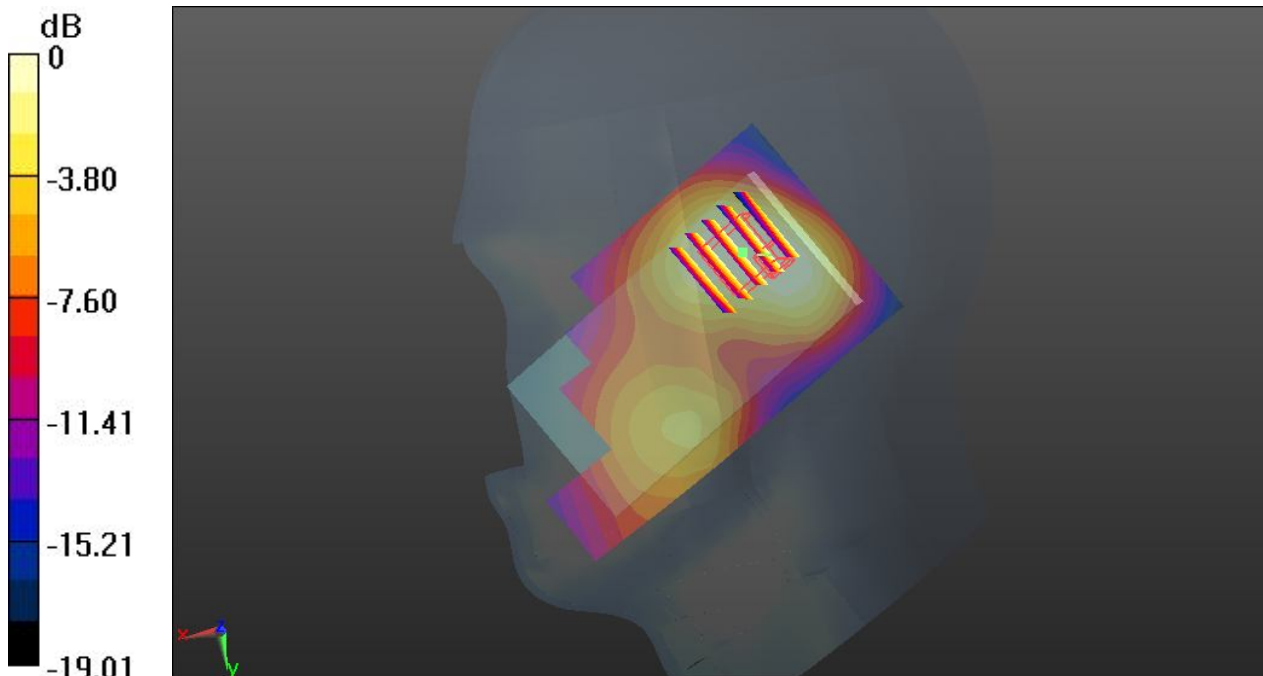
0 dB = 0.276 W/kg
