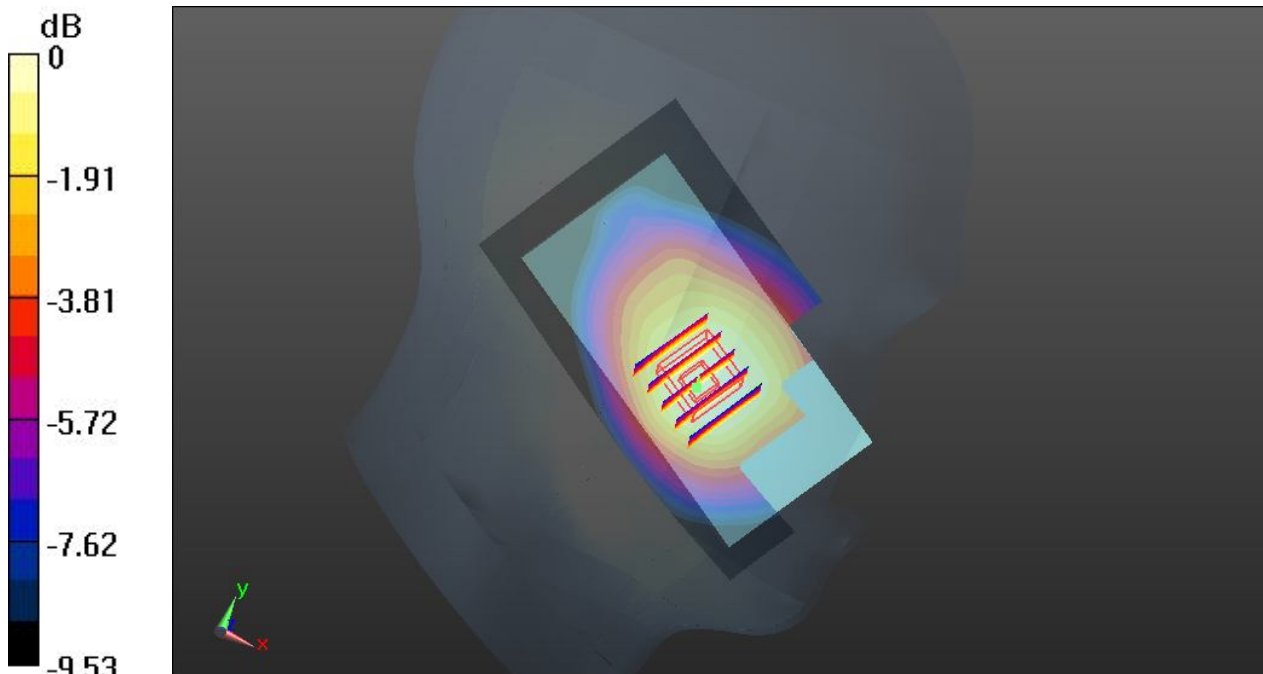
0 dB = 0.675 W/kg
