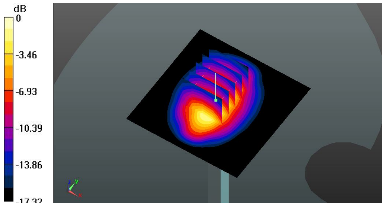
0 dB = 14.5 W/kg
