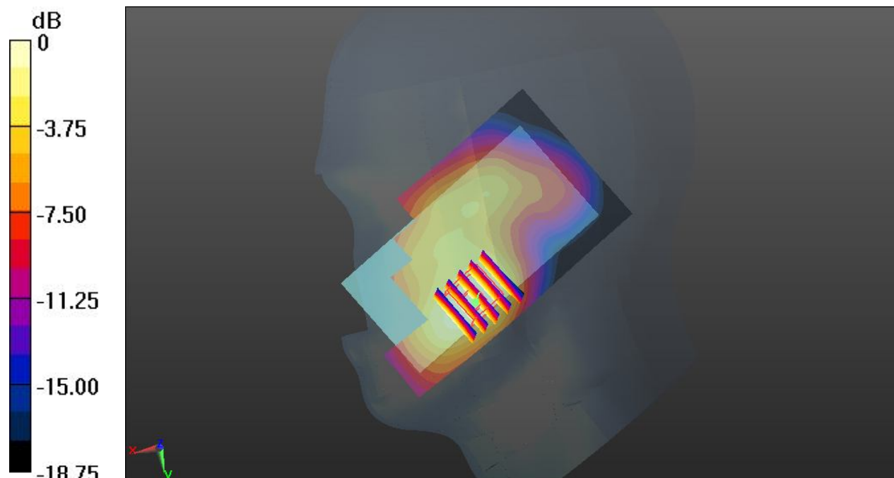
0 dB = 0.490 W/kg
