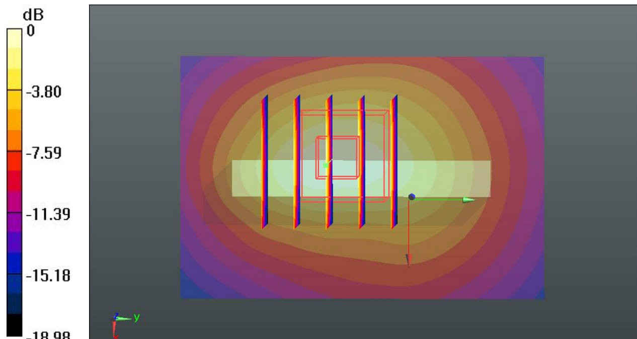
0 dB = 1.20 W/kg
