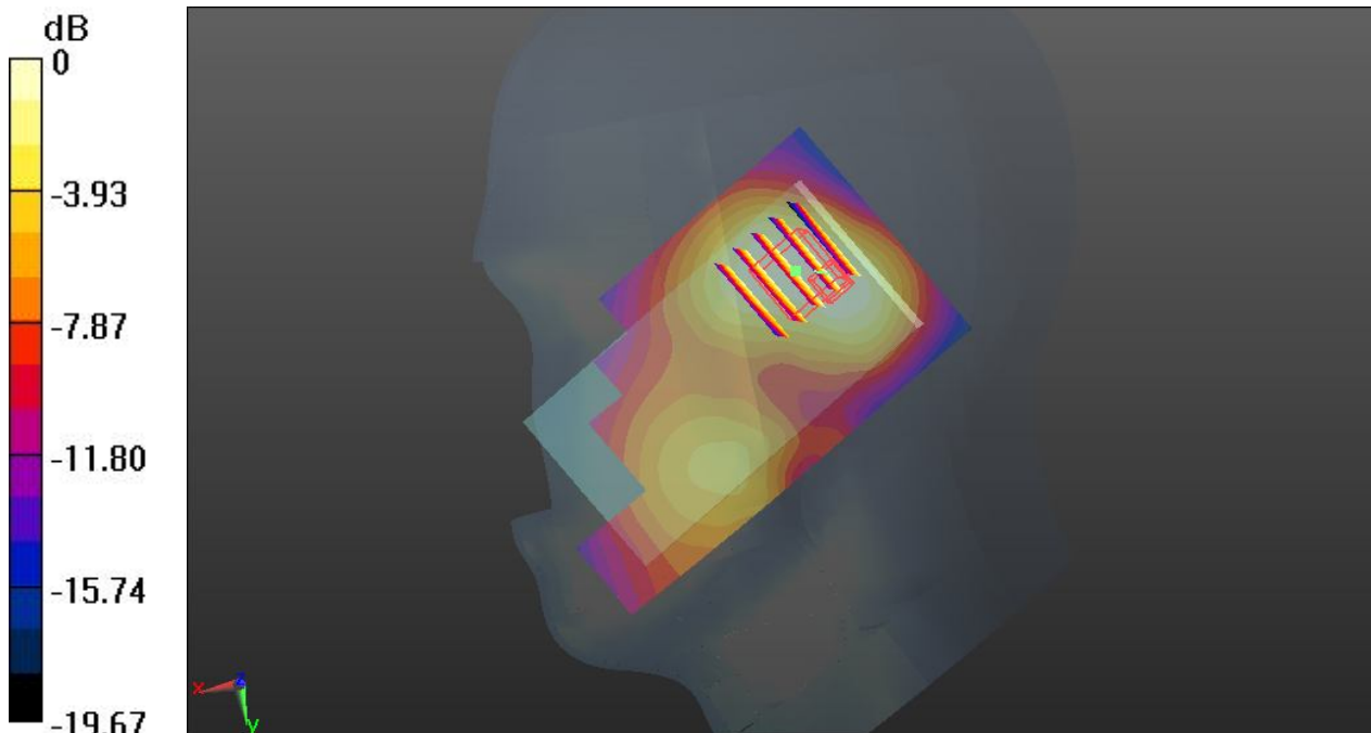
0 dB = 0.196 W/kg
