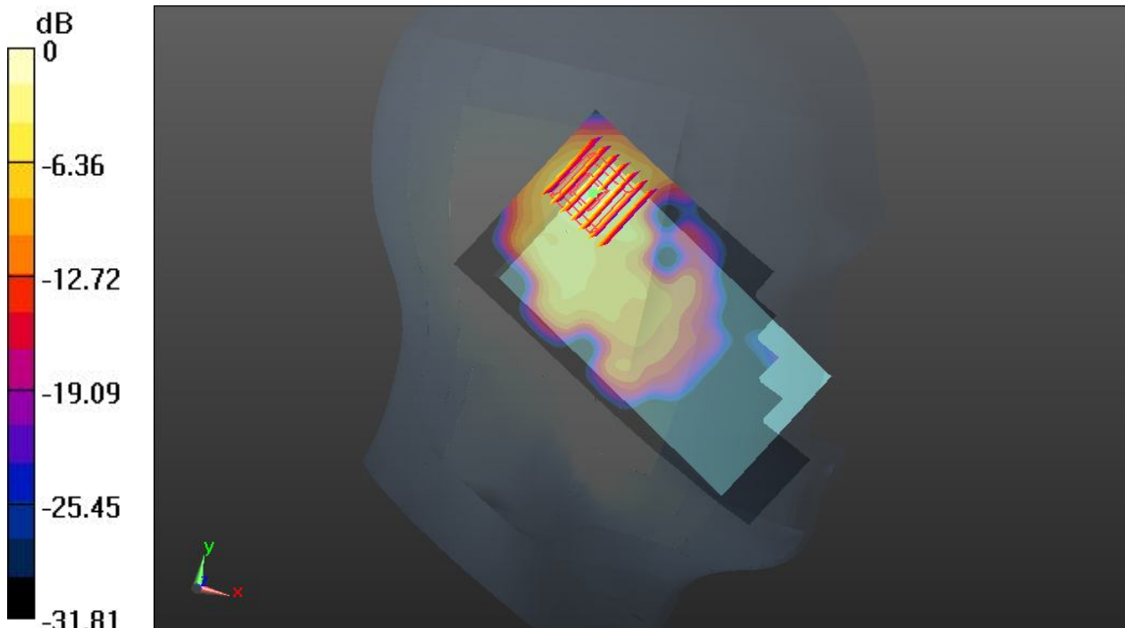
0 dB = 0.122 W/kg
