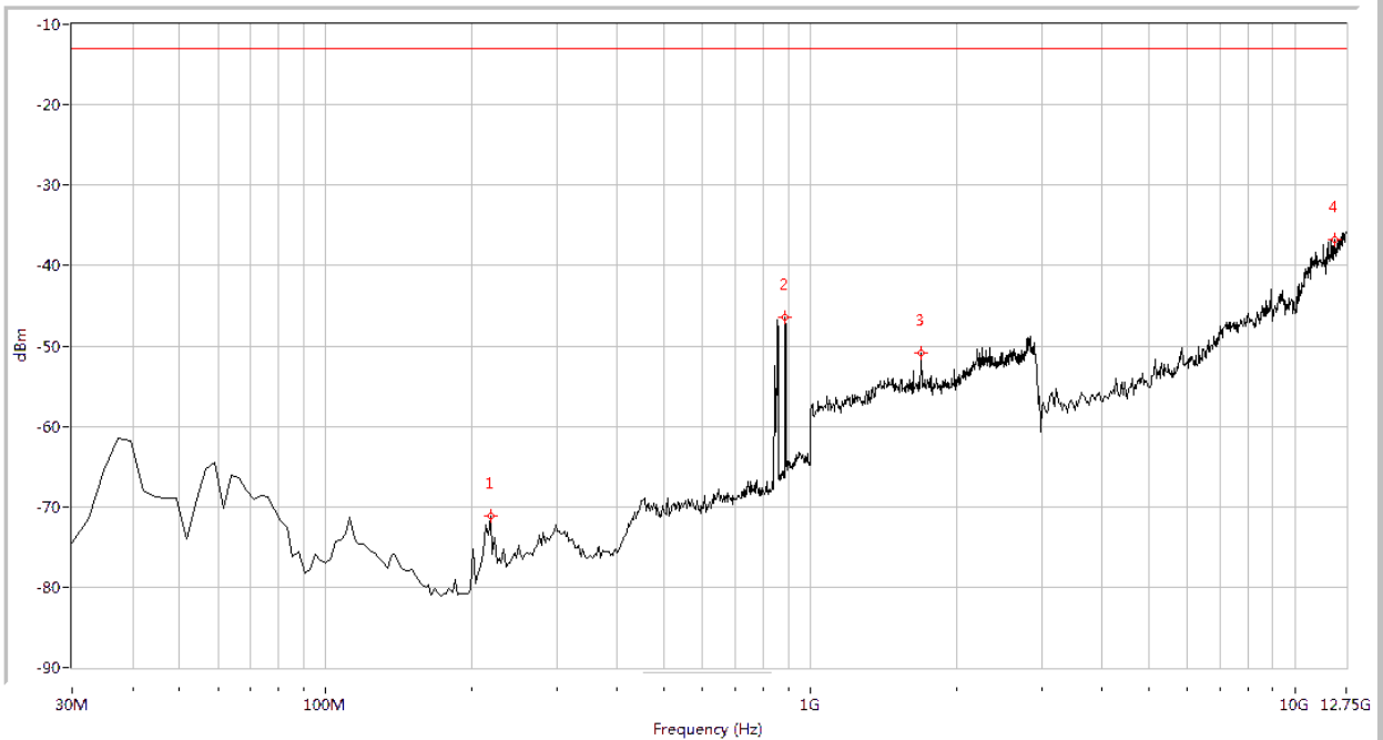
(Plot I.5: HSUPA 850MHz Channel = 4233, Test Antenna Horizontal)
