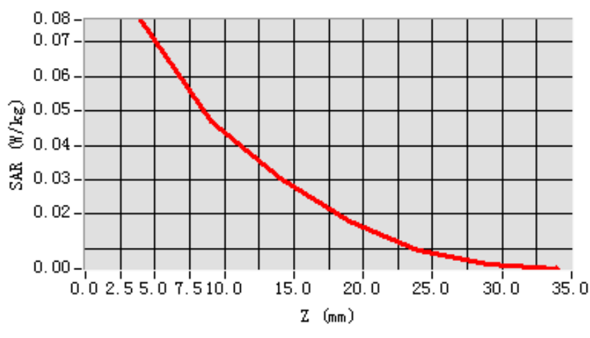
SAR, Z Axis Scan (X = -63, Y = -31)
