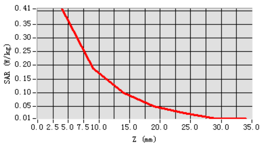
SAR, Z Axis Scan (X = 15, Y = 38)
