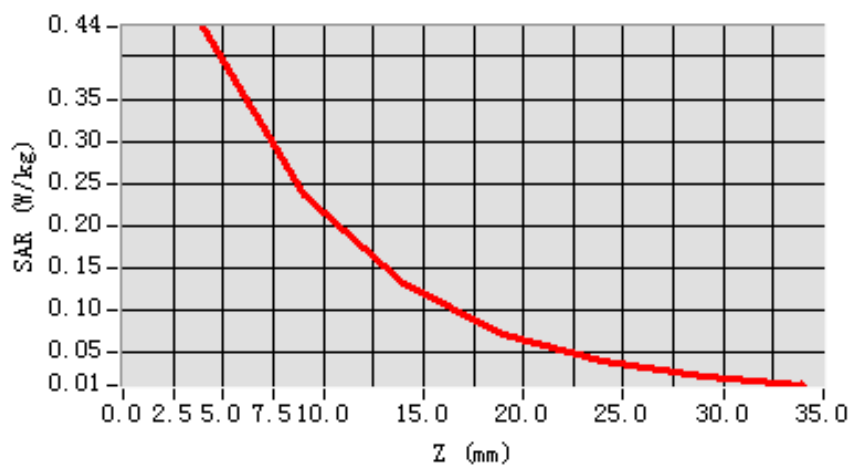
SAR, Z Axis Scan (X = -57, Y = -60)
