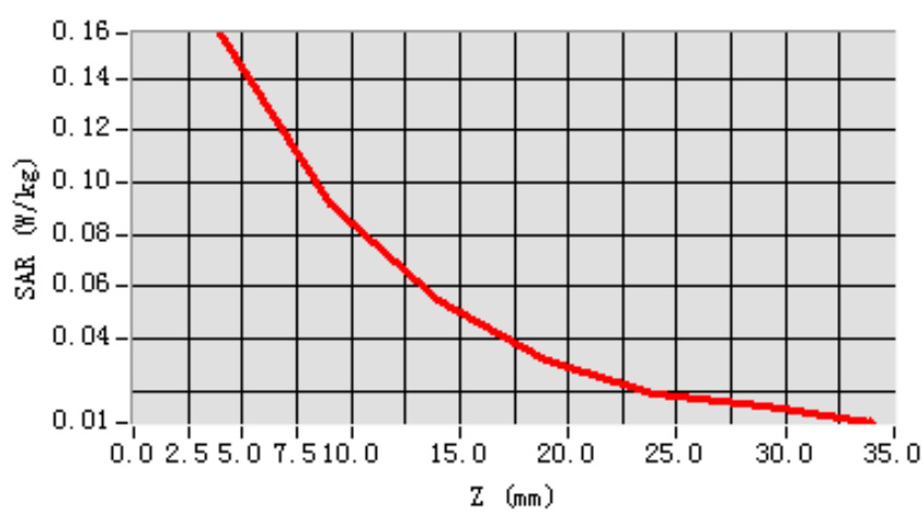
SAR, Z Axis Scan (X = 3, Y = 28)
