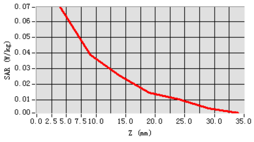
SAR, Z Axis Scan (X = -54, Y = -49)
