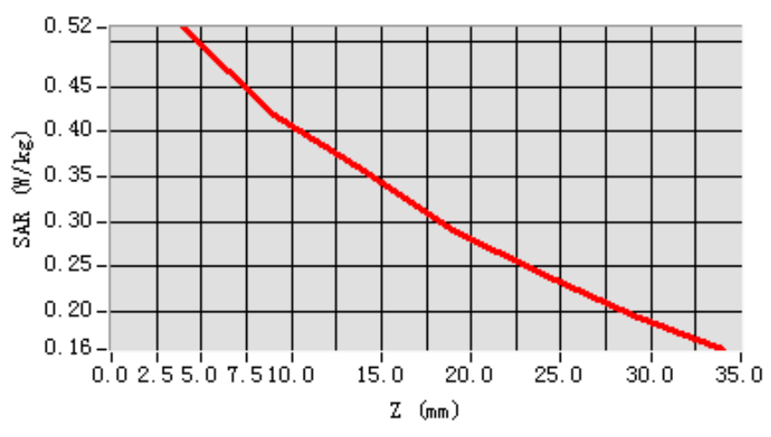
SAR, Z Axis Scan (X = -32, Y = -21)
