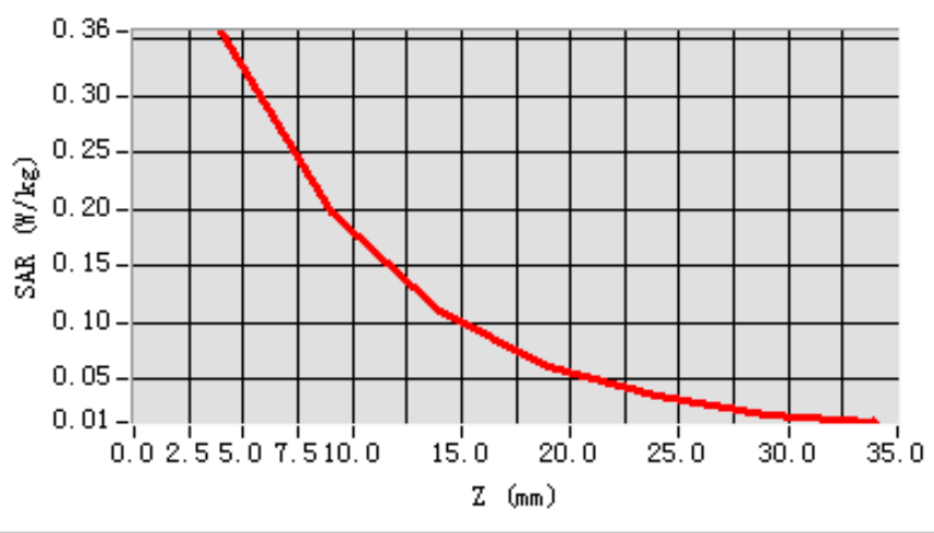
SAR, Z Axis Scan (X = -50, Y = -62)
