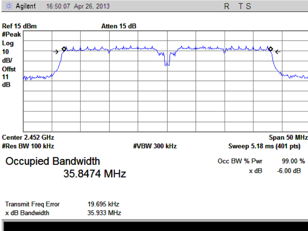
(Plot I: Channel 9: 2452MHz @ 802.11n-40)
