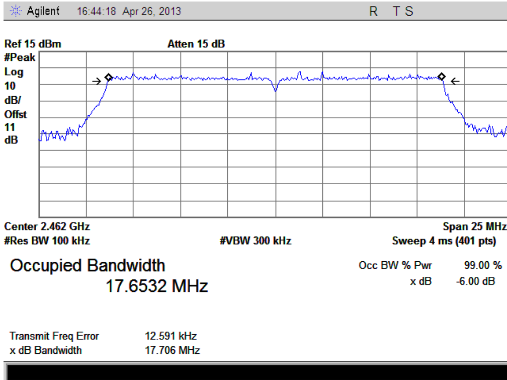
(Plot I: Channel 11: 2462MHz @ 802.11n-20)
