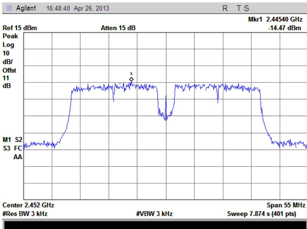
(Plot L: Channel = 9 @ 802.11n-40MHz)
