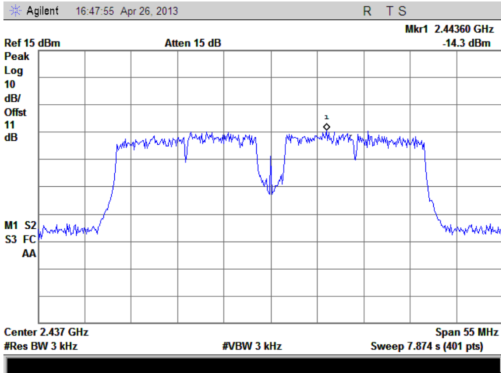
(Plot K: Channel = 6 @ 802.11n-40MHz)
