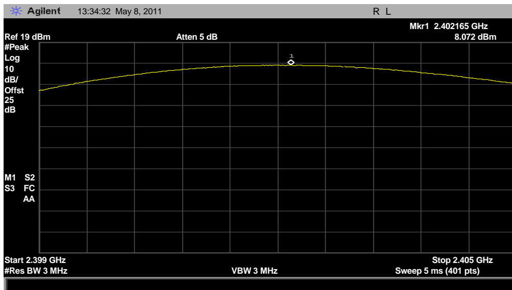
(Plot D: Channel = 2402)
