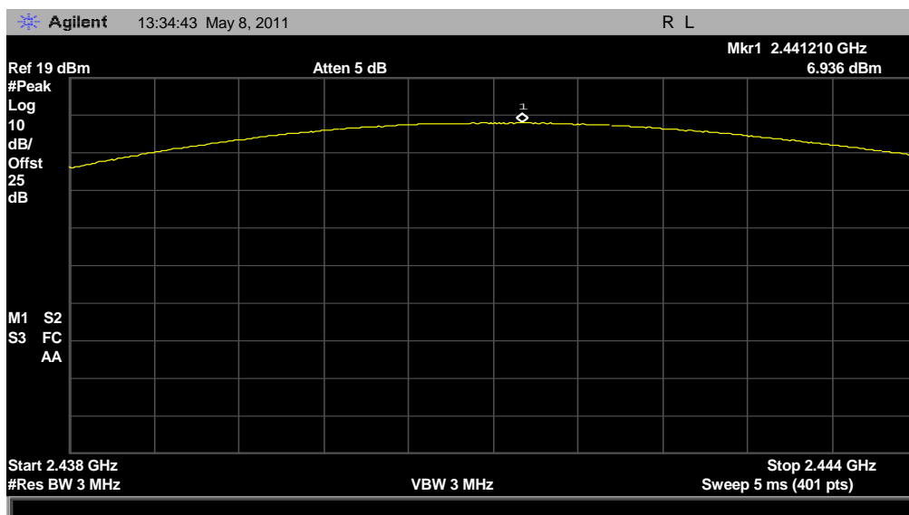
(Plot E: Channel = 2441)
