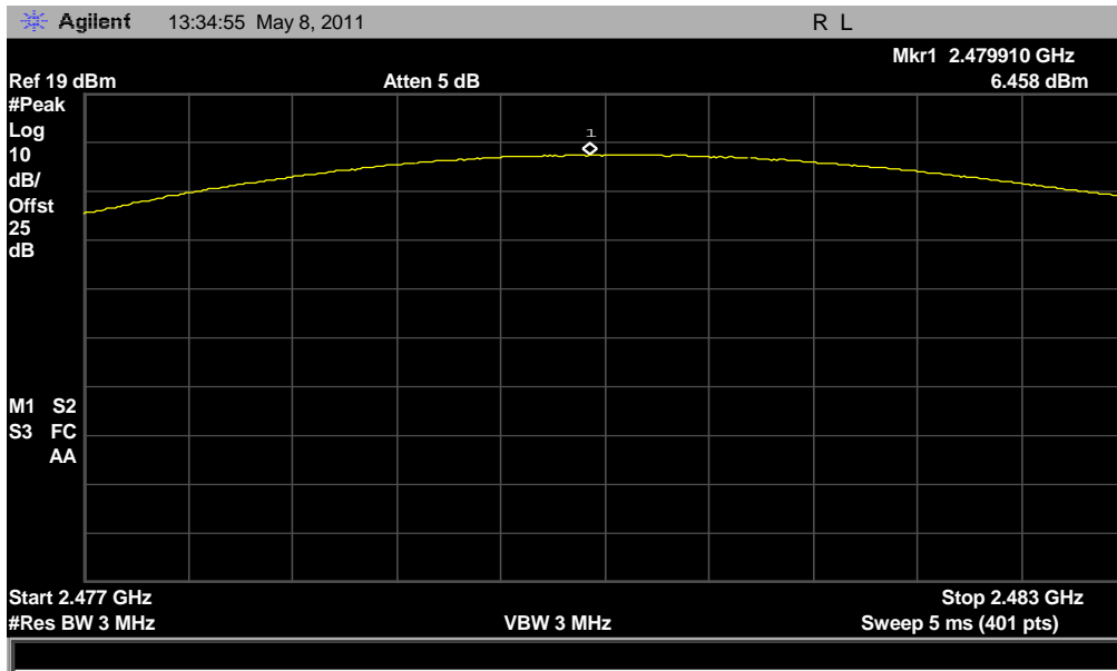
(Plot F: Channel = 2480)
