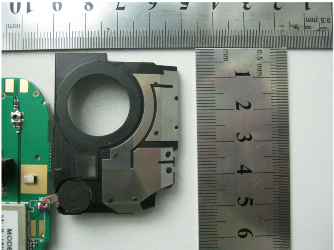
Primary Antenna
