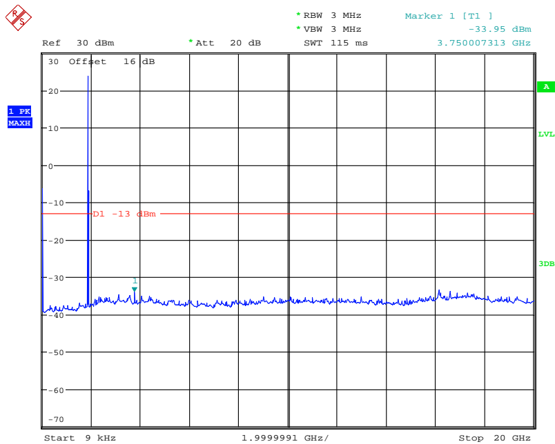
(Plot A4: WCDMA II Channel = 9662, 9KHz to 20GHz)
