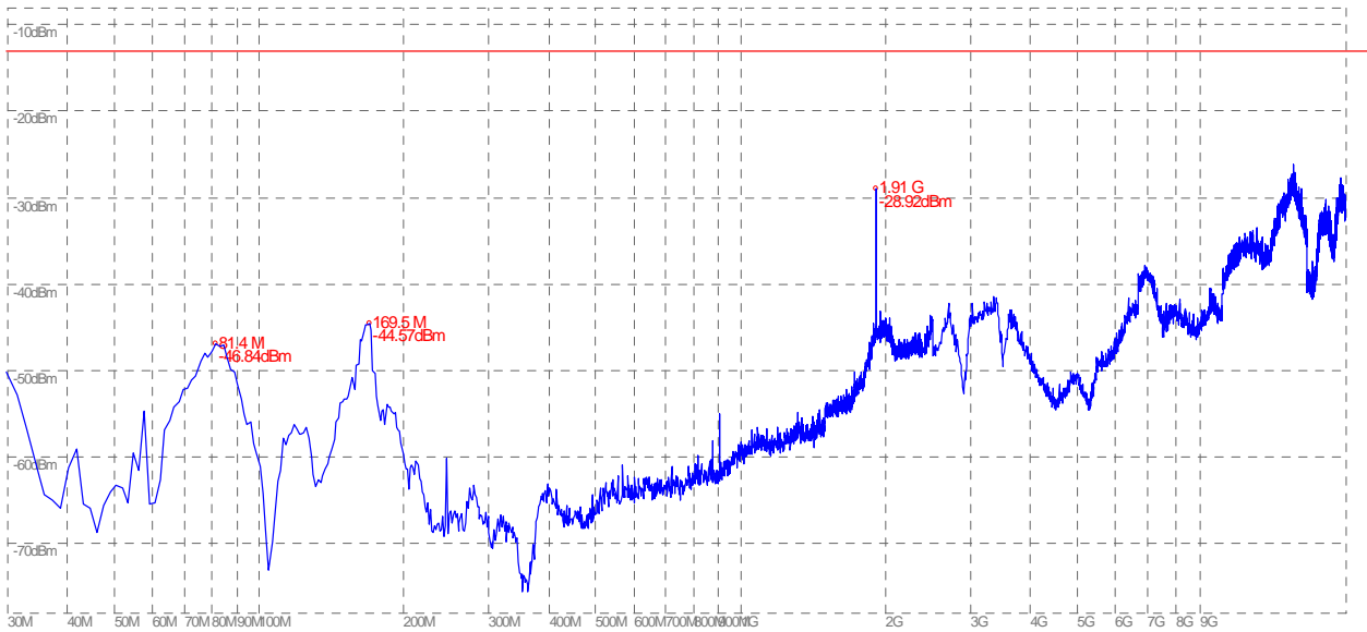
(Plot B.6: GSM 1900MHz Channel = 810, Test Antenna Vertical)
