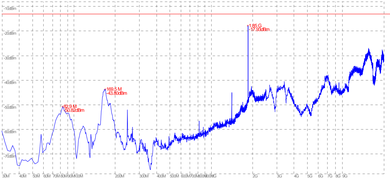
(Plot B.1: GSM 1900MHz Channel = 512, Test Antenna Horizontal)
