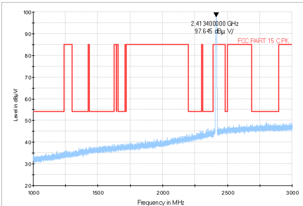
Fig.142 Radiated emission: Ch1, 1GHz-3GHz
