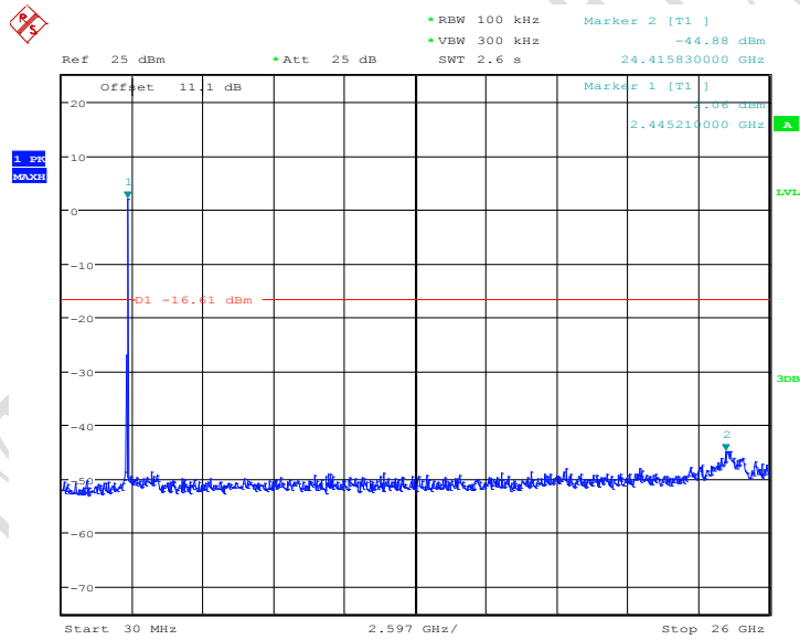
Fig.133 Conducted spurious emission: Ch11,1n,2462MHz
