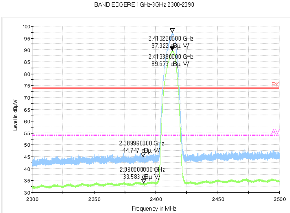
Fig.109 Frequency Band Edge: Ch1,11b
