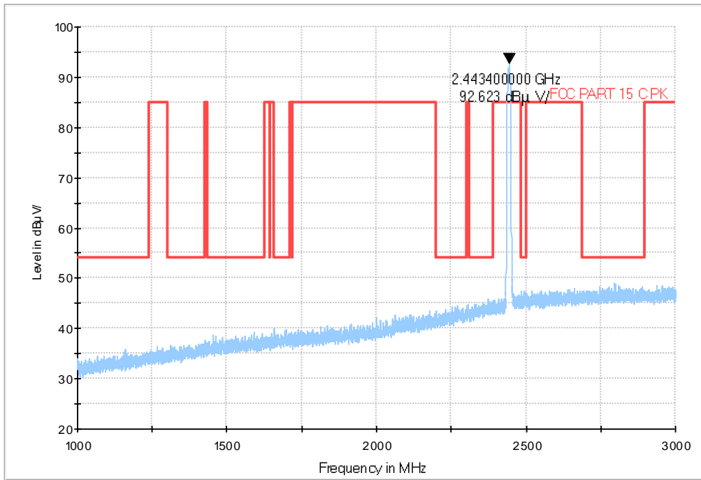
Fig.145 Radiated emission: Ch6, 1GHz-3GHz
