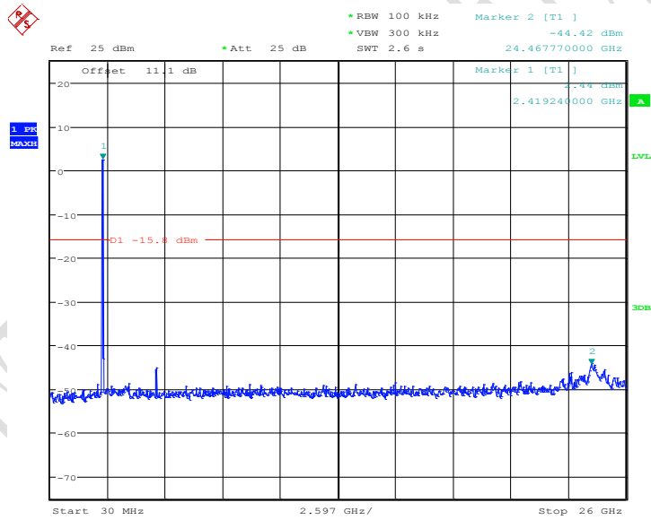
Fig.129 Conducted spurious emission: Ch1,11n,2412MHz
