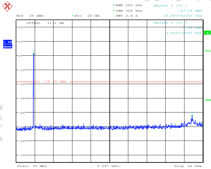
Fig.131 Conducted spurious emission: Ch6,11n,2437MHz
