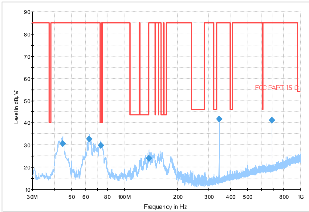
Fig.147 Radiated emission: Ch11, 30MHz-1GHz
