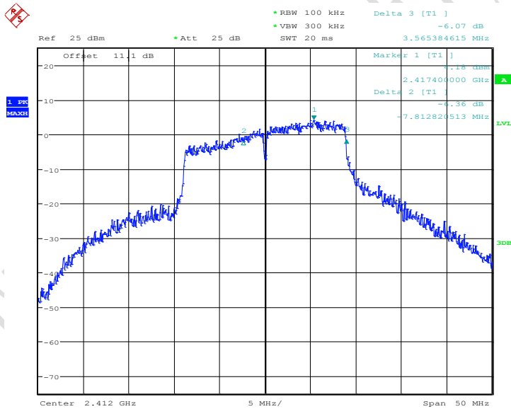
Fig.98 6dB Bandwidth: Ch1,11g
