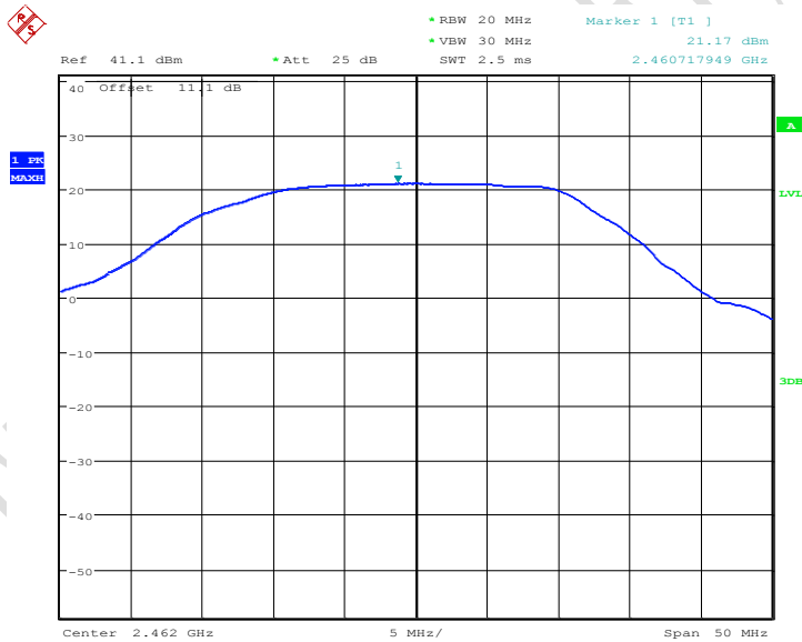
Fig.25 Conducted Output Power CH11, 11b, Rate1
