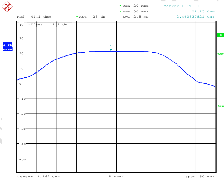
Fig.27 Conducted Output Power CH11, 11b, Rate5.5
