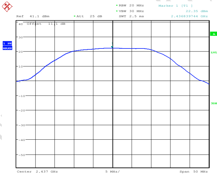
Fig.13 Peak Conducted Output Power CH6, 11b, Rate1
