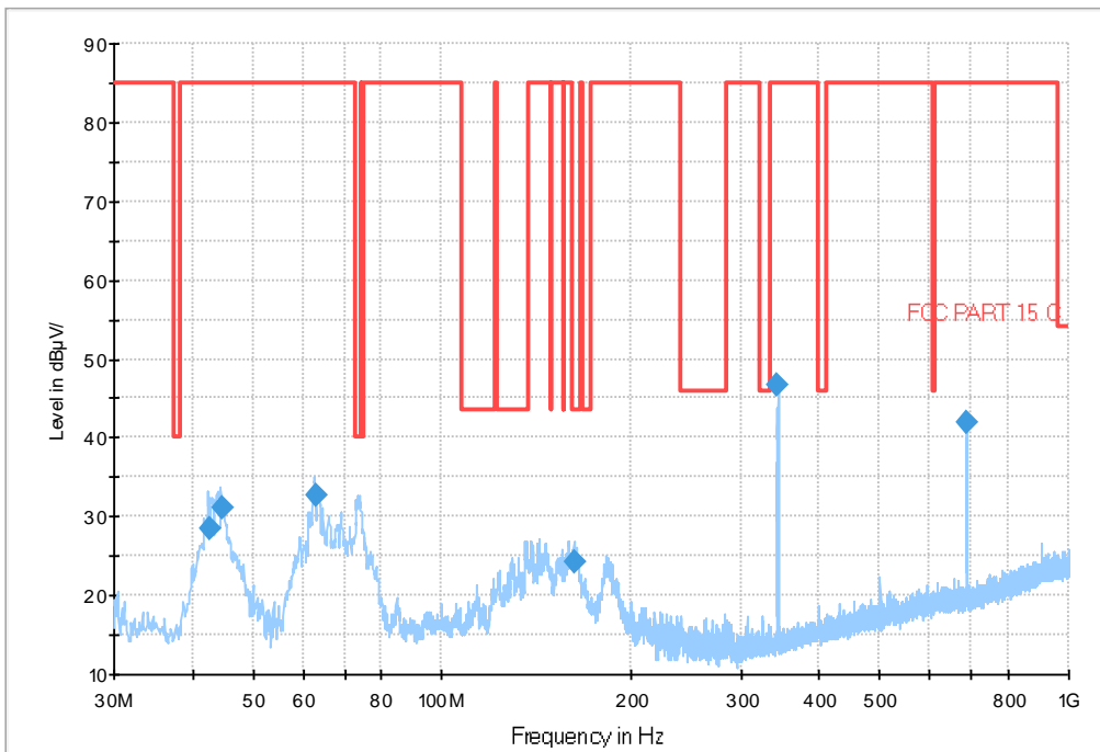
Fig.144 Radiated emission:Ch6, 30MHz-1GHz
