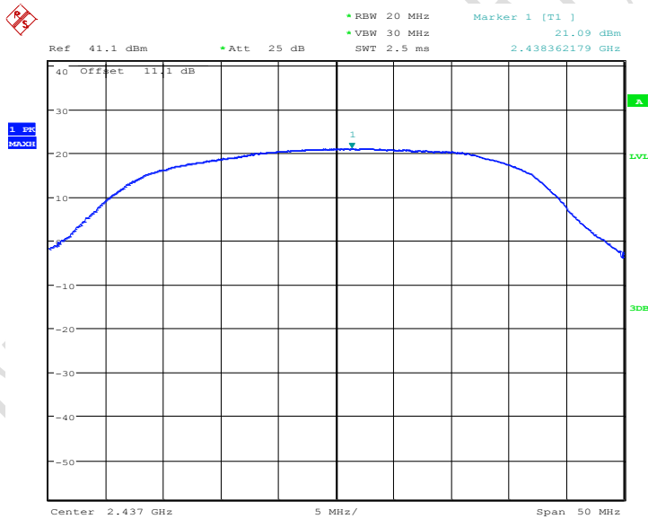
Fig.47 Conducted Output Power CH6, 11n, Rate MCS2
