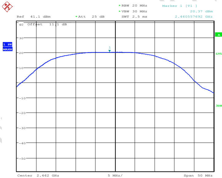
Fig.33 Conducted Output Power CH11, 11g, Rate24
