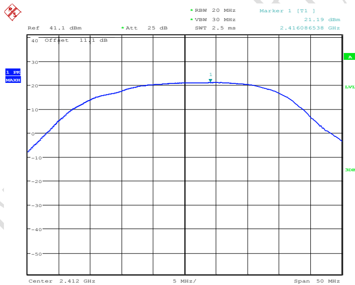
Fig.5 Peak Conducted Output Power CH1, 11g, Rate6
