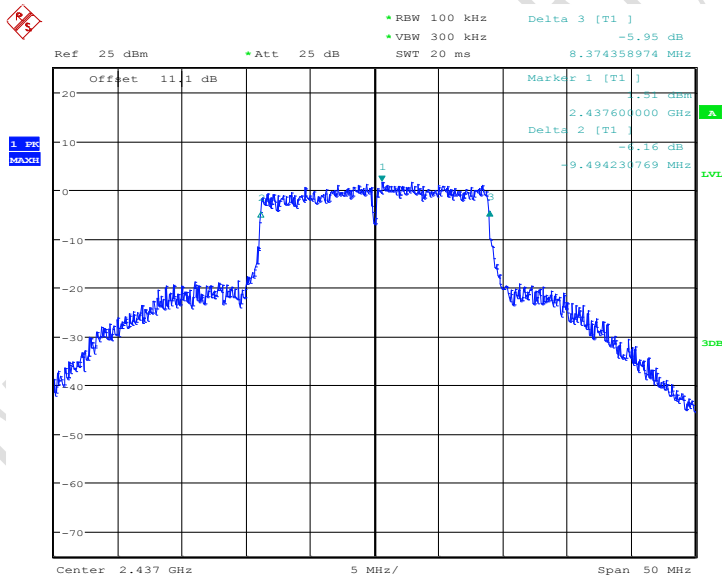
Fig.102 6dB Bandwidth: Ch6,11g
