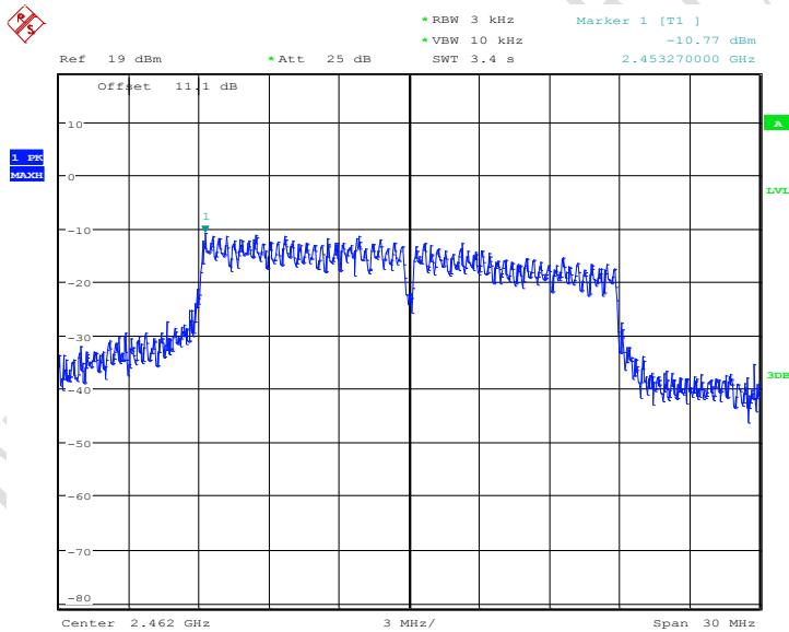
Fig.94 Power spectral density: CH11,11g
