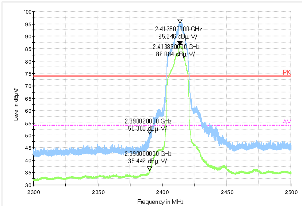
Fig.111 Frequency Band Edge: Ch1,11g
