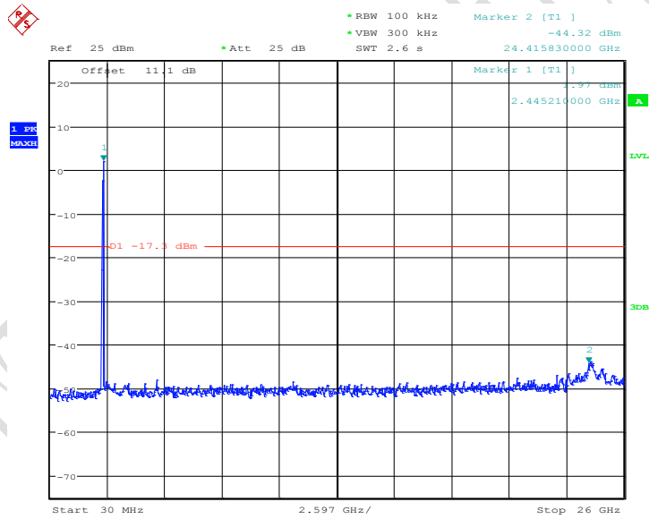
Fig.137 Conducted spurious emission: Ch6,11n(40M),2442MHz
