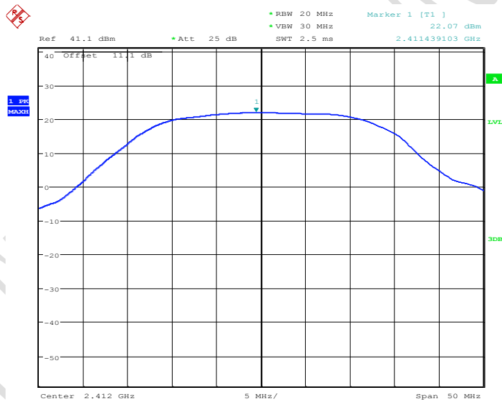
Fig.1 Peak Conducted Output Power CH1, 11b, Rate1
