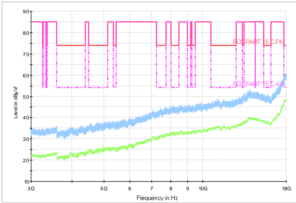
Fig.149 Radiated emission: Ch11, 3GHz-18GHz
