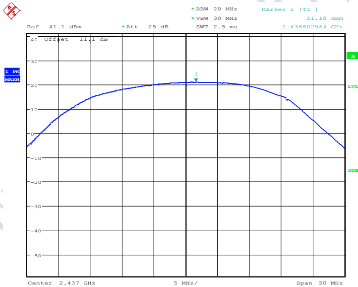
Fig.21 Conducted Output Power CH6, 11g, Rate24
