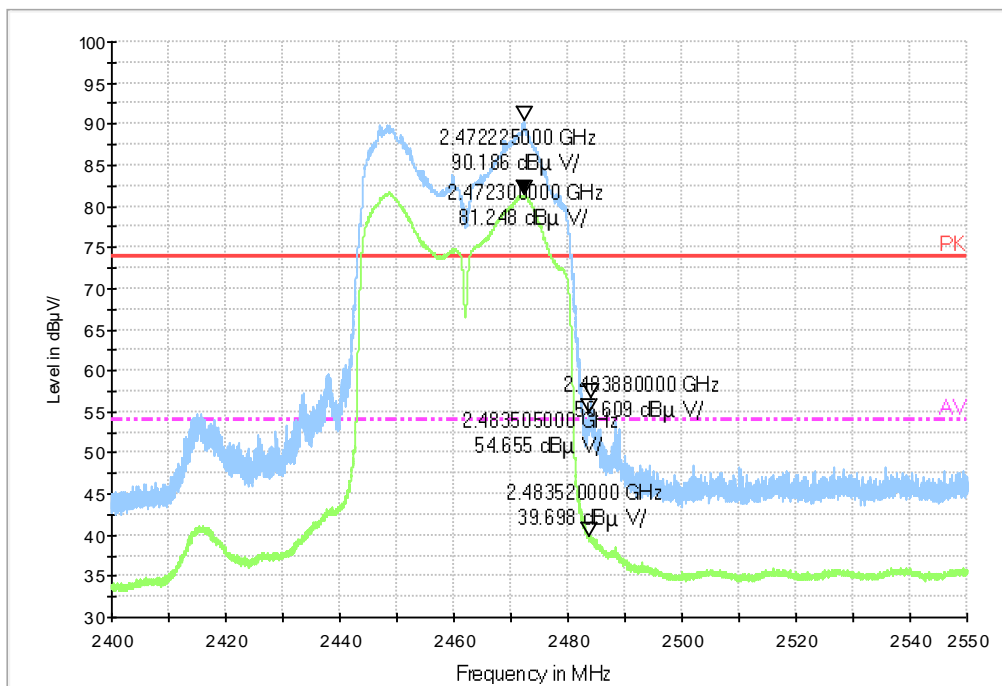
Fig.116 Frequency Band Edge: Ch9,11n(40M)
