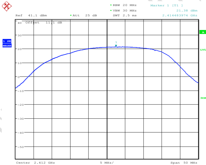
Fig.9 Peak Conducted Output Power CH1, 11g, Rate24
