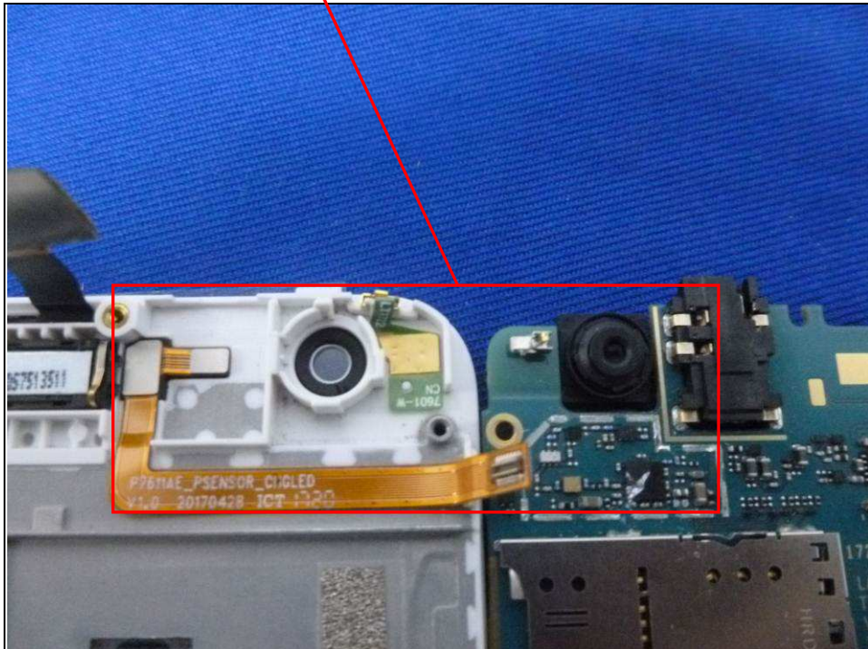
BT/WLAN Antenna
