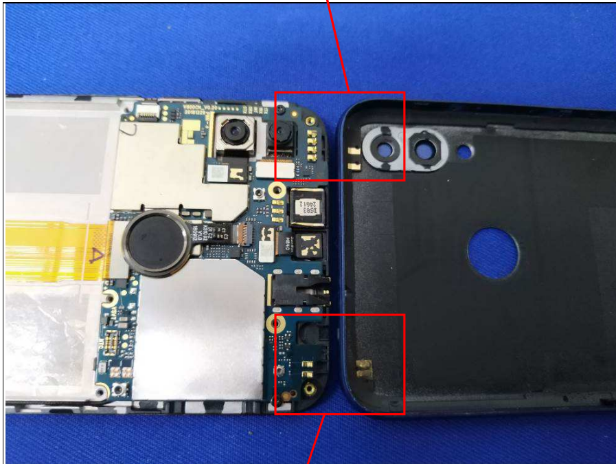
BT/WLAN/GPS Antenna
