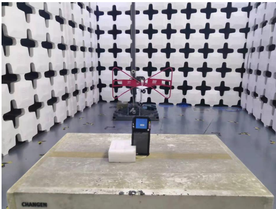
10. Radiated Emissions (Part 15C Wi-Fi/Bluetooth, 30MHz-1GHz)
