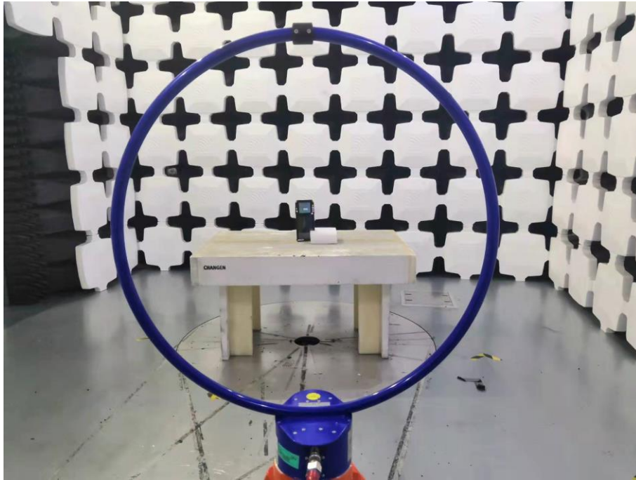
9. Radiated Emissions (Part 15C Wi-Fi/Bluetooth, 9kHz-30MHz)
