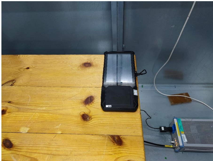
16. Conducted Emission (Part 15C, Wi-Fi/Bluetooth)
