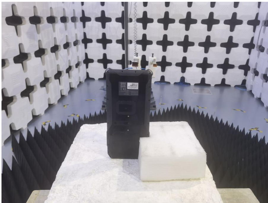
12. Radiated Emissions (Part 15C Wi-Fi/Bluetooth, 18GHz -26.5GHz)
