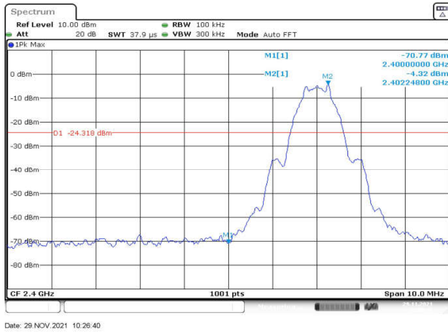
Fig.7 Band Edges (Ch 0), LE 1M
