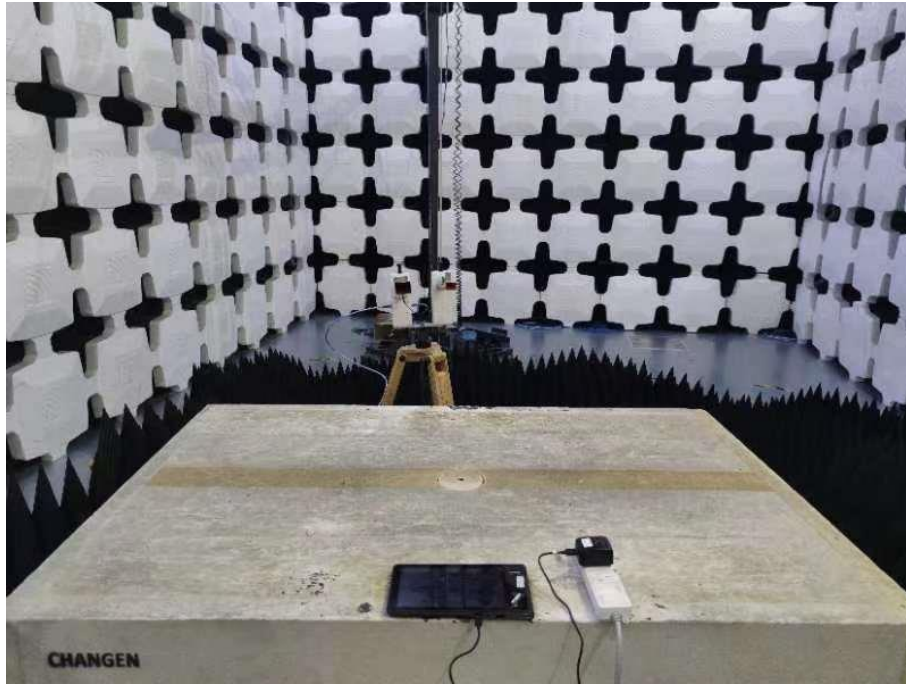
11. Radiated Emissions (Part 15B, Camera, 18GHz-26.5GHz)
