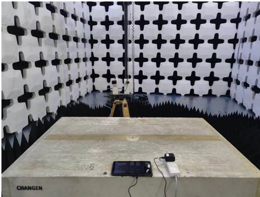
12. Radiated Emissions (Part 15B, Camera, 26.5GHz-40GHz)
