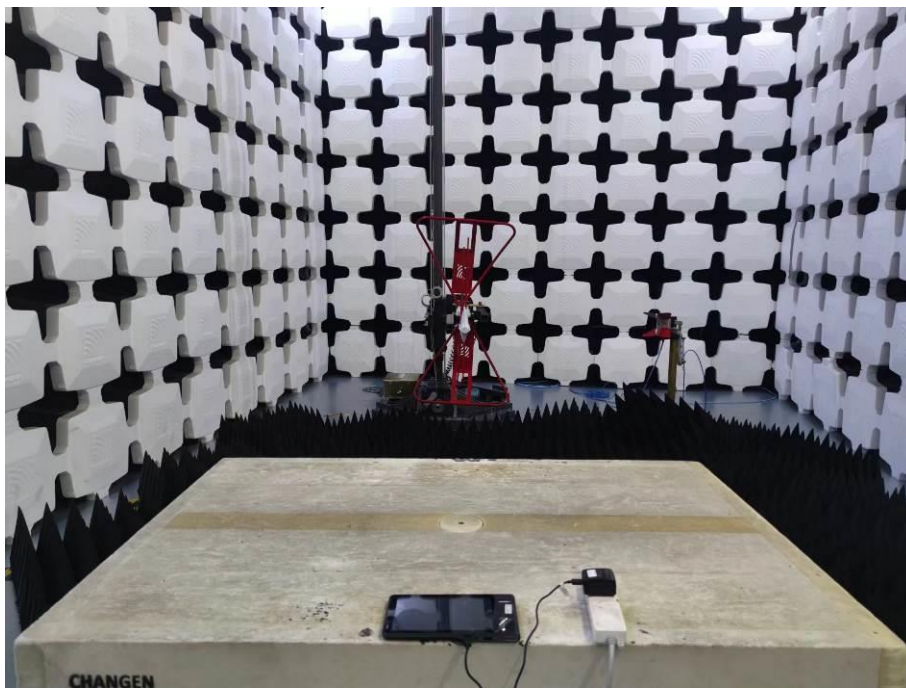
10. Radiated Emissions (Part 15B, Camera,1GHz-18GHz)
