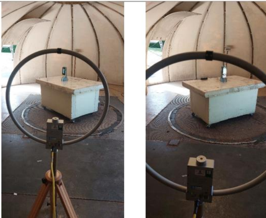
Photo of Field strength within the band 13.110-14.010MHz in OATS
