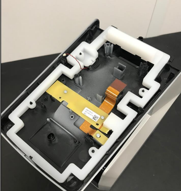
TOP LCD and PCB
