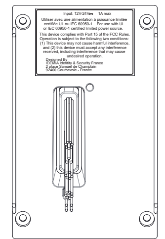
Ratings, FCC and manufacturer address Label (location on equipped trap door)
