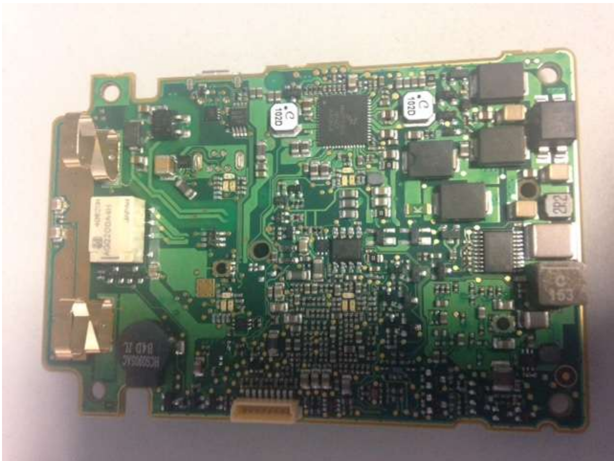
Motherboard (BOTTOM)
