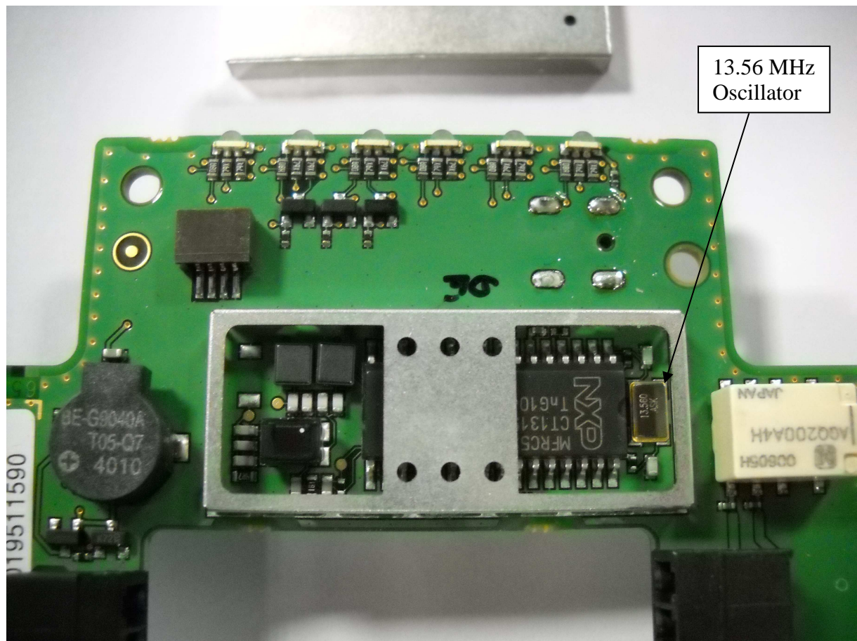
Printed board 1 side A with metallic cover removed
