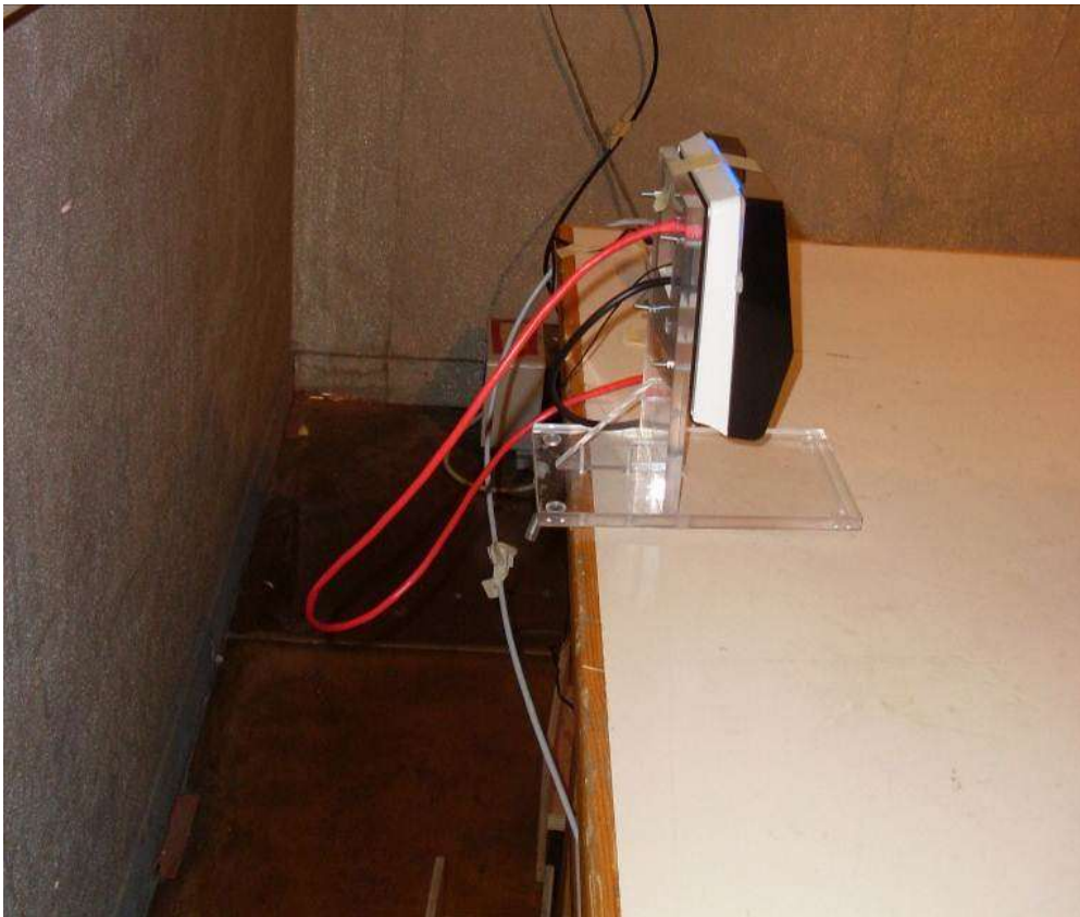
Test setup for power line conducted emissions (POE adaptor)
