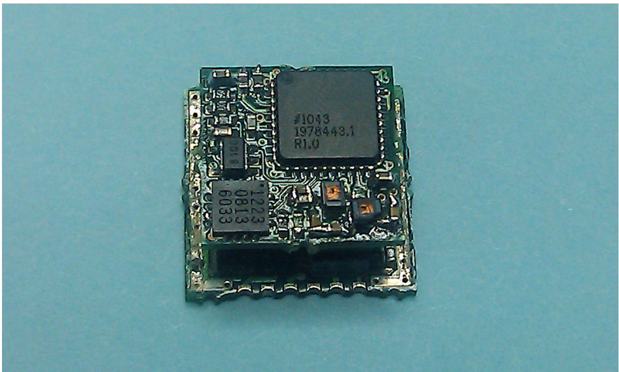
Photo 5 Transmitter Module, Shield Removed
