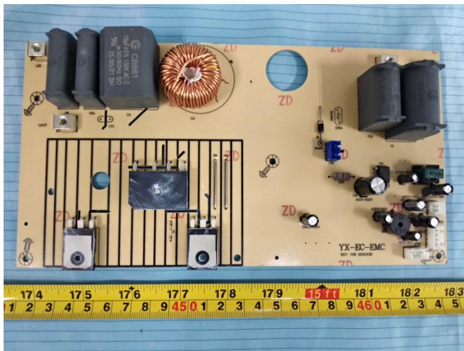
EUT –Power Board Top Shielding off View
