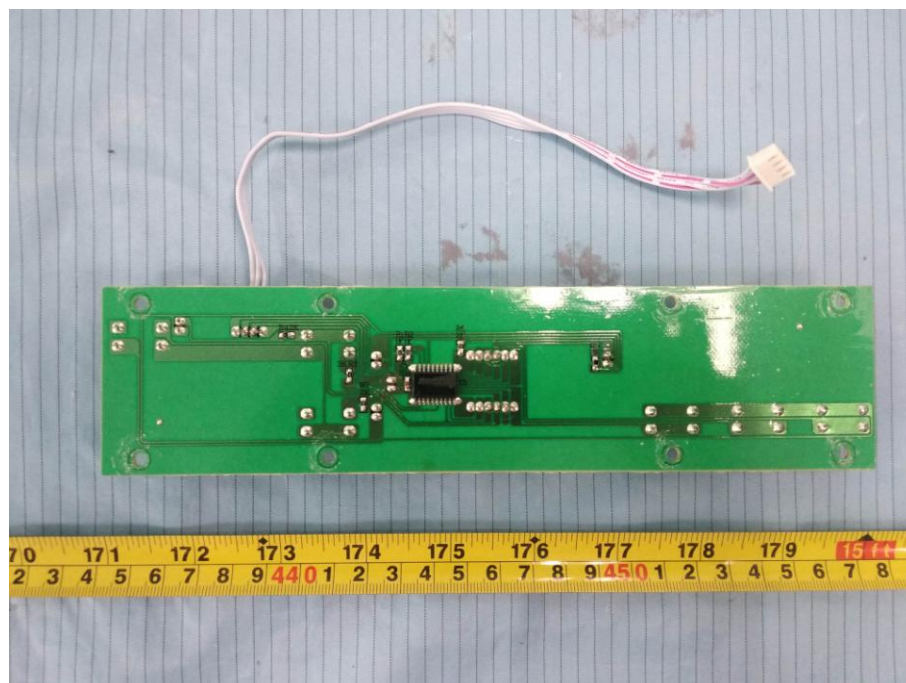
EUT –Keypad Board Board Bottom View
