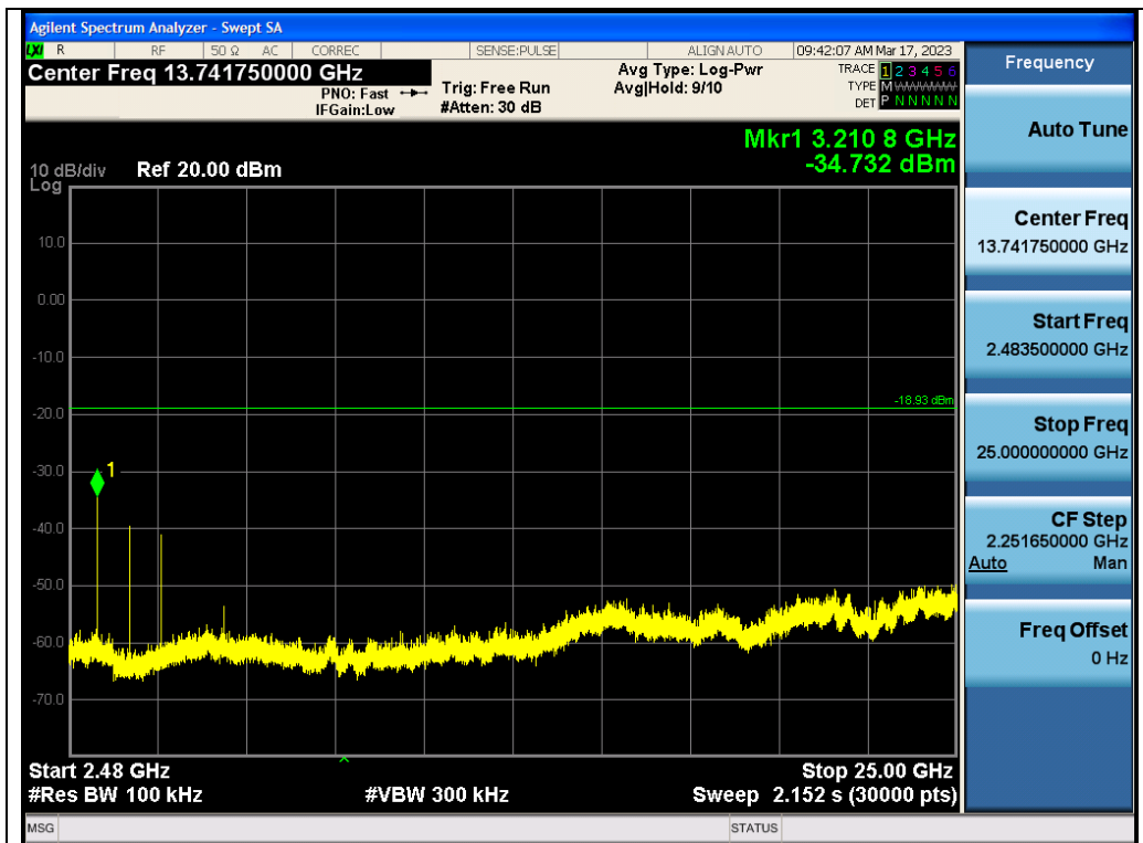
Test_Graph_GFSK_ANT1_2408_Higher Band Emissions
