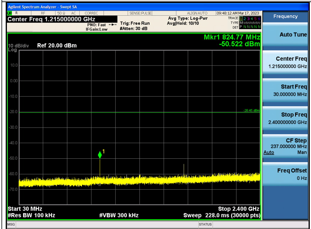
Test_Graph_GFSK_ANT1_2474_Lower Band Emissions
