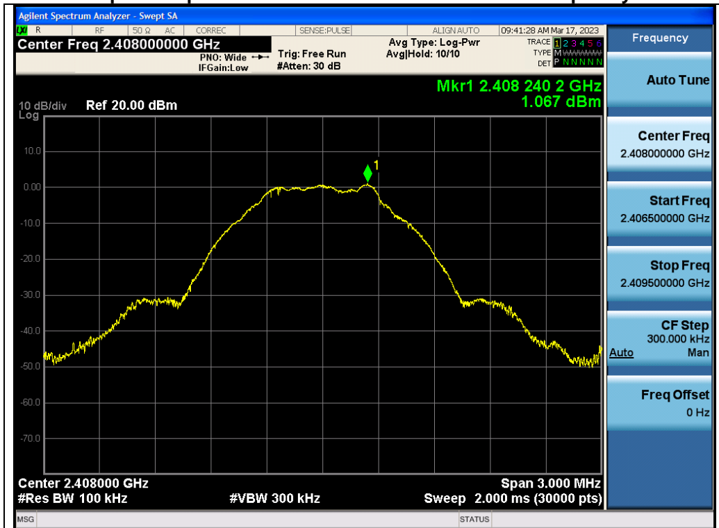
Test_Graph_GFSK_ANT1_2408_Reference Level
