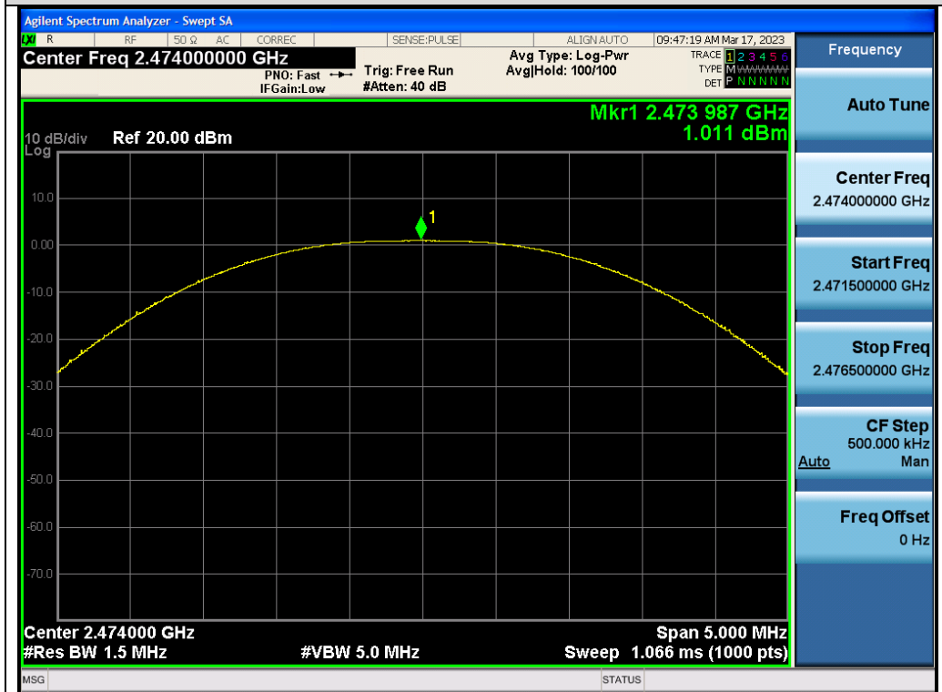
Test_Graph_GFSK_ANT1_2474_Peak Power
