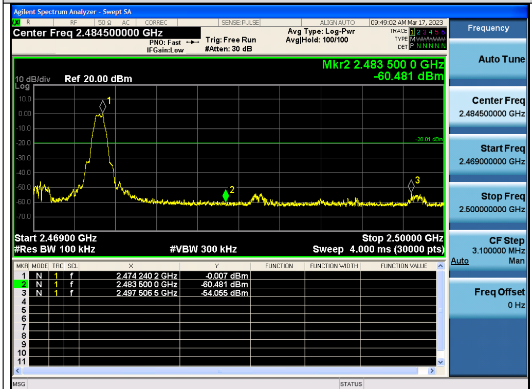
Test_Graph_GFSK_ANT1_2474_Higher Band Edge Emissions
