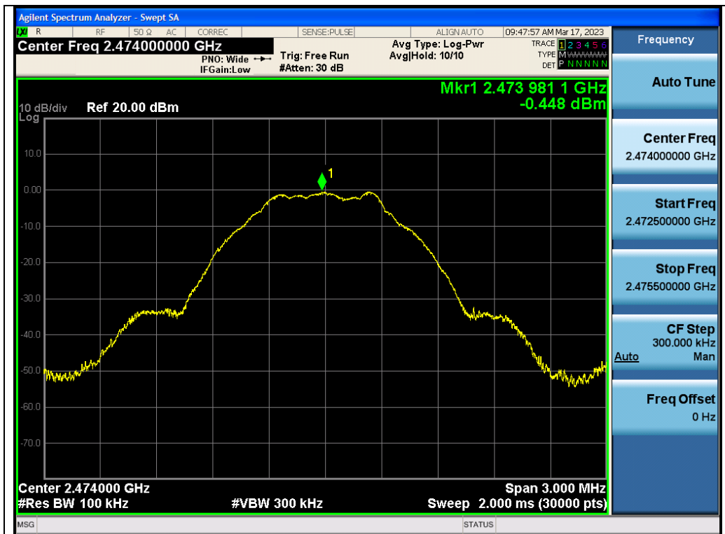
Test_Graph_GFSK_ANT1_2474_Reference Level
