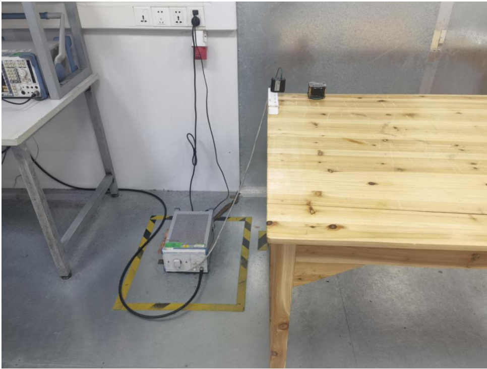
FCC ID:ZBCWD268A Photo of Conducted Emission Measurement
