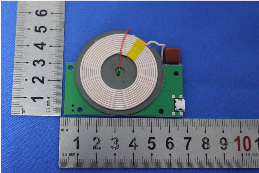
Model: WD-210AA (for SMD NTC)
