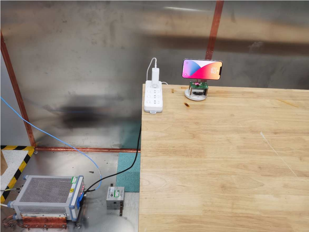
Photograph 3: Set-up photo for Conducted Emission (Apple Magsafe+Wireless Charger)
