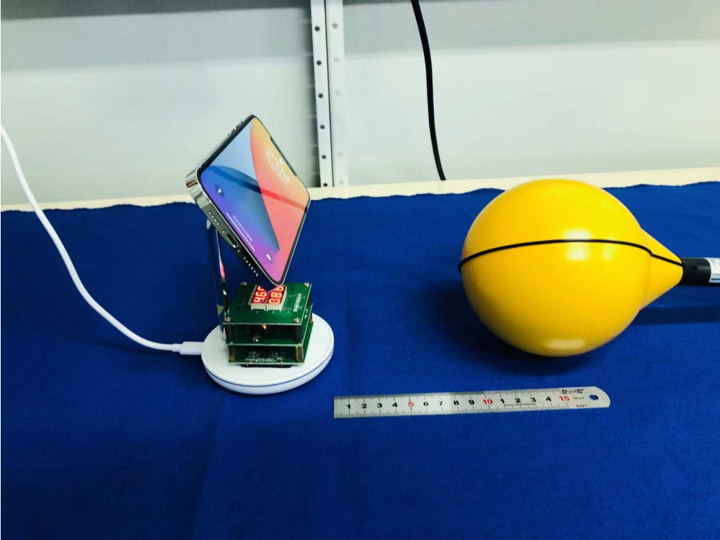
Photograph 5: Set-up photo for RF Exposure(Apple Magsafe+Wireless Charger)
