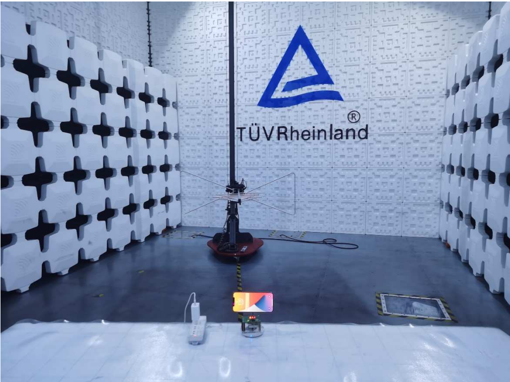
Photograph 4: Set-up photo for Radiated Emission (Apple Magsafe+Wireless Charger)
