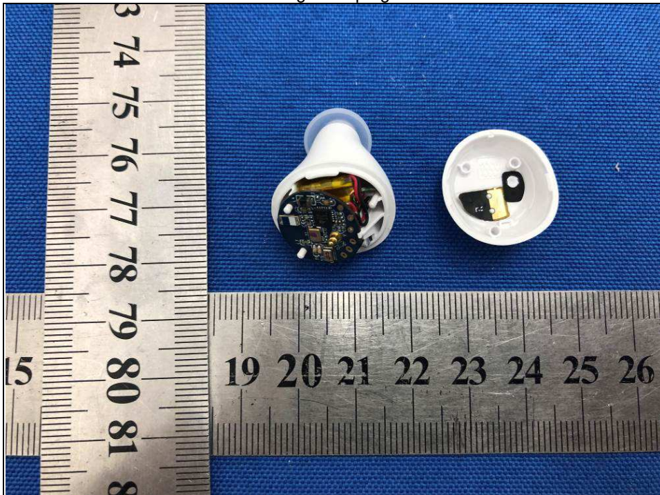
Right Earplug
