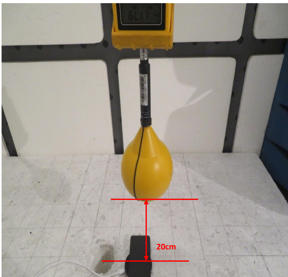
TestPosition E-Exposure photo from top surface(20cm)
