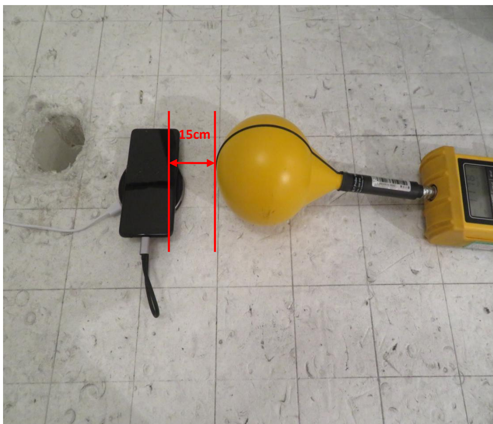
TestPosition D-Exposure photo from side edge surface-Right
