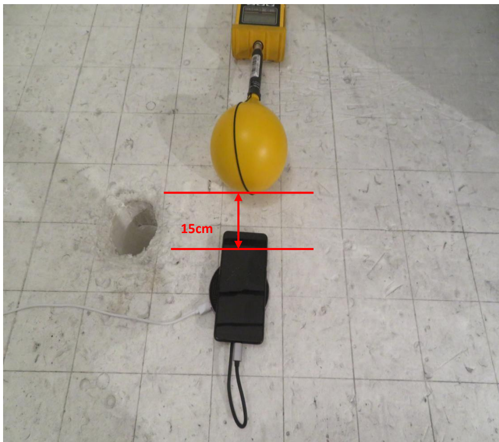
TestPosition C-Exposure photo from side edge surface-Front
