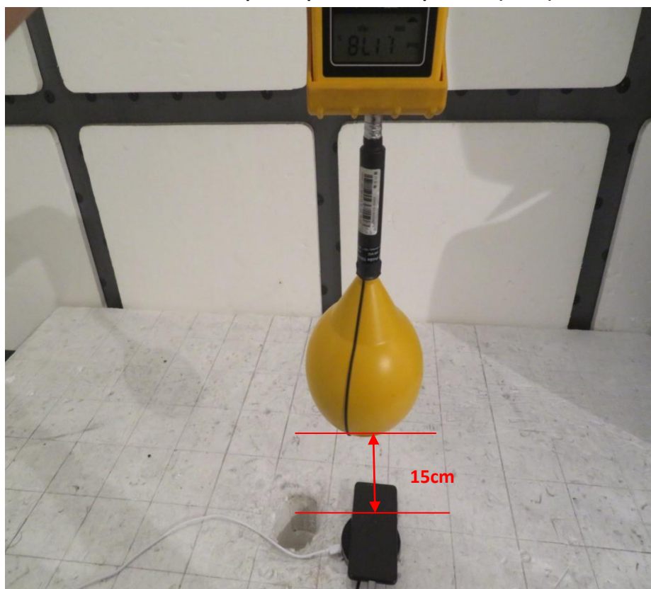
TestPosition E-Exposure photo from top surface(15cm)
