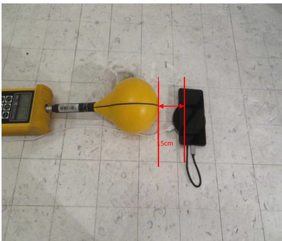
TestPosition B-Exposure photo from side edge surface-Left
