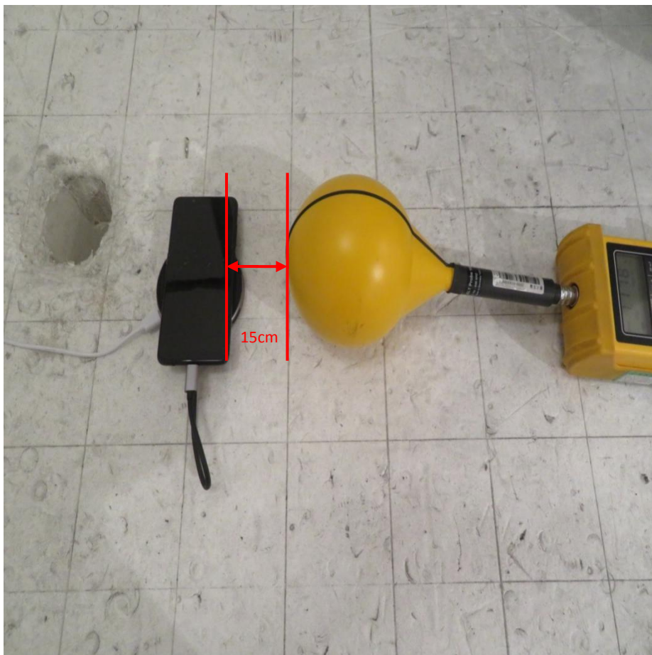
TestPosition A-Exposure photo from side edge surface-Rear
