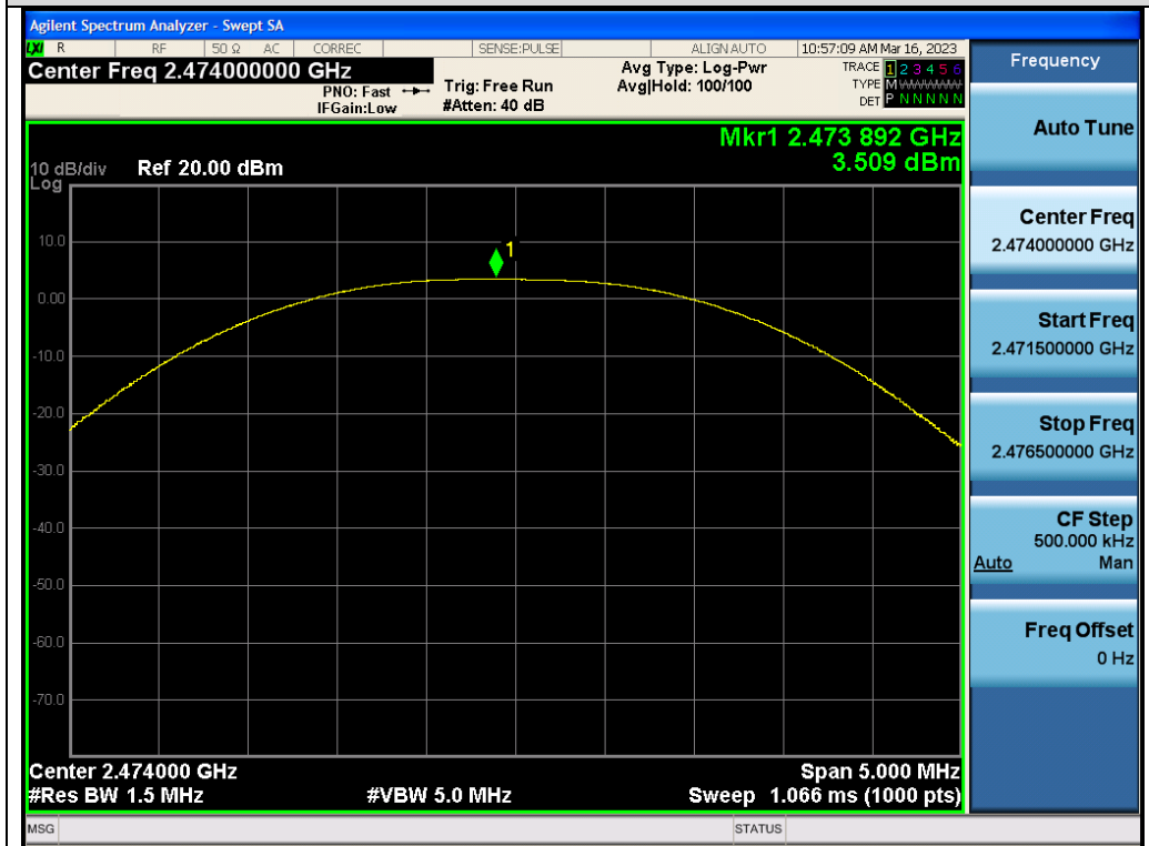
Test_Graph_GFSK_ANT1_2474_Peak Power
