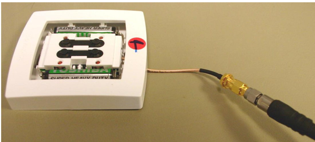
Photo . Detail test set-up conducted emission
