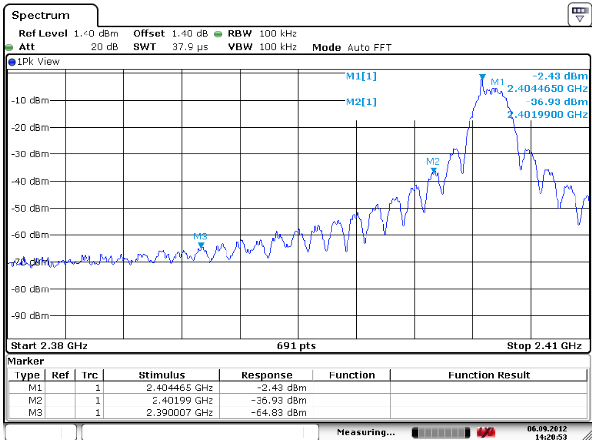
Figure 12: Band Edge Conducted Emission, Spectral Diagram, Mode A (2405MHz)
