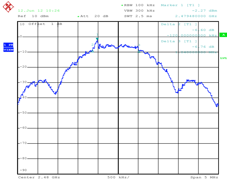
Figure 5: 6dB Bandwidth, Mode C (2480MHz)
