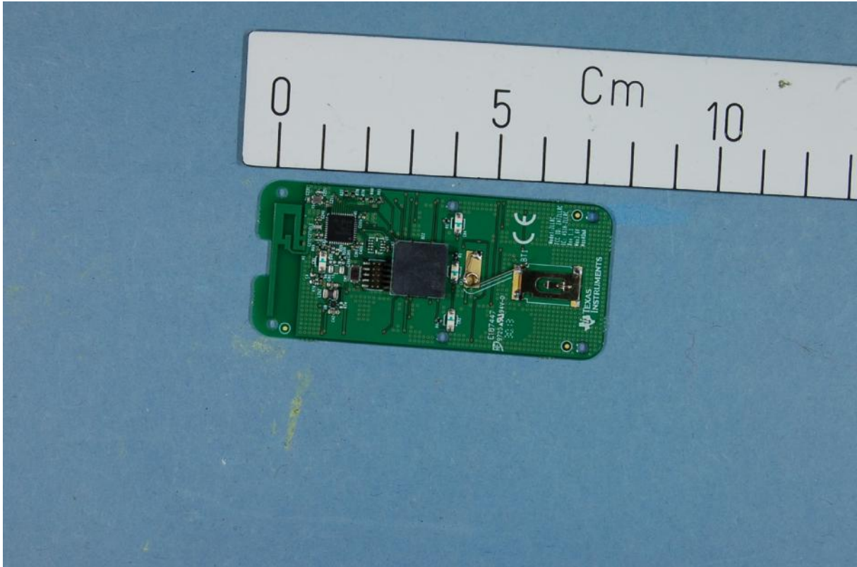
ZLLRC – PCB component side
