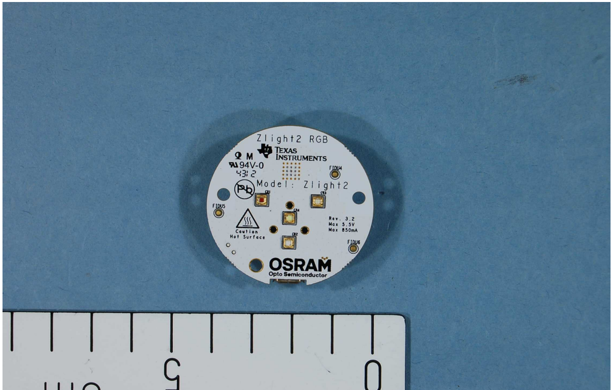
Zlight2, EUT for radiated measurements
