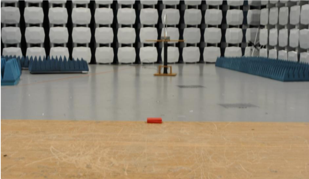
Radiated emissions - < 30MHz, 10 meter
