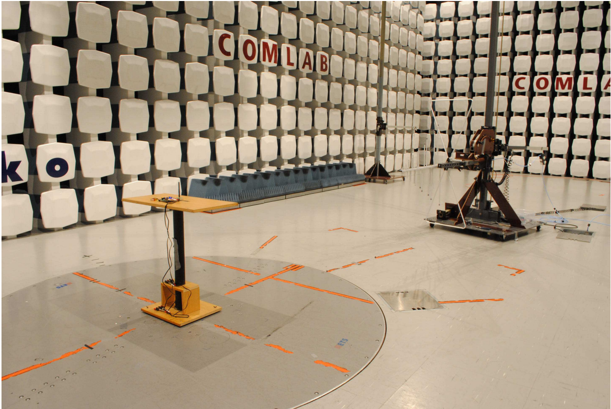
Radiated Emissions
