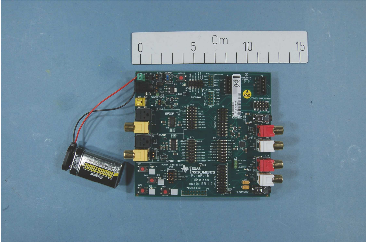
Evaluation board – Front
